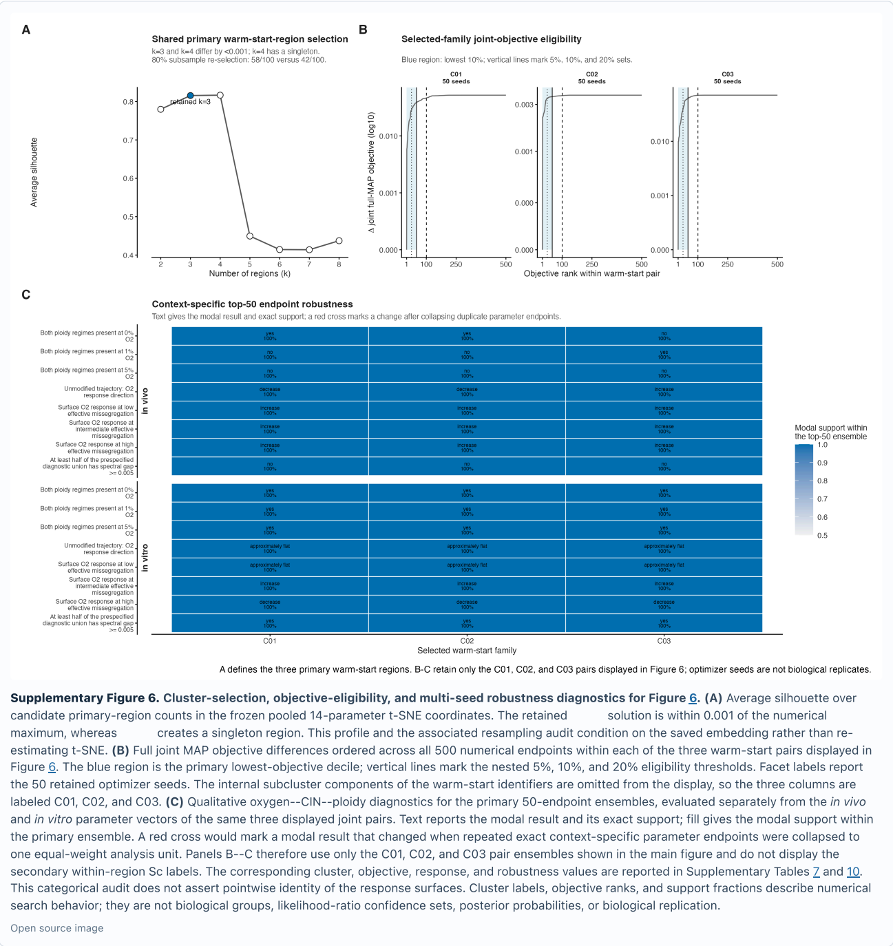
Supplementary Figure 6. Cluster-selection, objective-eligibility, and multi-seed robustness diagnostics for Figure 6. (A) Average silhouette over candidate primary-region counts in the frozen pooled 14-parameter t-SNE coordinates. The retained solution is within 0.001 of the numerical maximum, whereas creates a singleton region. This profile and the associated resampling audit condition on the saved embedding rather than re-estimating t-SNE. (B) Full joint MAP objective differences ordered across all 500 numerical endpoints within each of the three warm-start pairs displayed in Figure 6. The blue region is the primary lowest-objective decile; vertical lines mark the nested 5%, 10%, and 20% eligibility thresholds. Facet labels report the 50 retained optimizer seeds. The internal subcluster components of the warm-start identifiers are omitted from the display, so the three columns are labeled C01, C02, and C03. (C) Qualitative oxygen--CIN--ploidy diagnostics for the primary 50-endpoint ensembles, evaluated separately from the in vivo and in vitro parameter vectors of the same three displayed joint pairs. Text reports the modal result and its exact support; fill gives the modal support within the primary ensemble. A red cross would mark a modal result that changed when repeated exact context-specific parameter endpoints were collapsed to one equal-weight analysis unit. Panels B--C therefore use only the C01, C02, and C03 pair ensembles shown in the main figure and do not display the secondary within-region Sc labels. The corresponding cluster, objective, response, and robustness values are reported in Supplementary Tables 7 and 10. This categorical audit does not assert pointwise identity of the response surfaces. Cluster labels, objective ranks, and support fractions describe numerical search behavior; they are not biological groups, likelihood-ratio confidence sets, posterior probabilities, or biological replication.
