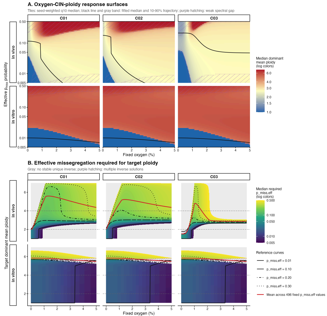
Figure 6. Paired joint-fit context vectors yield context- and family-dependent oxygen--CIN--ploidy responses. (A) Joint-fit oxygen--CIN--ploidy response surfaces. Columns show C01Sc01, C02Sc01, and C03Sc02, abbreviated C01, C02, and C03; rows show the context-specific in vivo and in vitro vectors from the same retained joint endpoints. Within each context--pair panel, the complete grid of 201 oxygen concentrations and 60 forced effective per-chromosome missegregation probabilities was evaluated for the 50 joint endpoints in the pair-specific lowest-objective decile. Fill reports seed-weighted median dominant mean ploidy in its original units; the color mapping is logarithmic and progresses from blue at low ploidy through yellow to red at high ploidy. Black curves show the pointwise median model-implied population-average missegregation probability along the unmodified context-specific fixed-O trajectories, and gray ribbons show their 10th--90th percentile intervals. Purple diagonal hatching and dotted boundaries identify grid cells where at least half of eligible endpoint vectors have ; white crosses mark sampled positions where fewer than 80% agree on whether dominant mean ploidy is at least 2. Exact duplicate 14-parameter vectors were evaluated once within each context and restored to their original optimizer-seed multiplicities before aggregation. These surfaces summarize numerical fit multiplicity in fitted context-specific parameterizations; they are not independently fitted CIN measurements, causal oxygen-by-CIN interventions, or biological confidence regions (Supplementary Figures 6 and 7; Supplementary Tables 7 and 10). (B) Context-specific inverse oxygen--ploidy maps with fixed-input reference trajectories. Endpoint-level dense curves were evaluated separately in both contexts at 496 forced probabilities from 0.005 through 0.500 in increments of 0.001 and numerically inverted over target dominant mean ploidy 1--7 in increments of 0.025. Where at least 80% of the seed-weighted endpoint vectors had exactly one inverse solution and fewer than 20% had multiple solutions, color shows the seed-weighted median returned by the piecewise-linear inverse; color spacing is logarithmic and labels remain in original probability units. Purple hatching marks cells where at least 20% of endpoints had multiple inverse solutions. Light gray marks cells without an ensemble-supported unique inverse in the evaluated probability interval, including targets that were not reached consistently. Black curves show the forward median-ploidy trajectories at fixed , 0.10, 0.20, and 0.30 using solid, dash--dot--dot, dot--dash, and dotted lines, respectively. At each oxygen concentration, the red solid curve is the arithmetic mean of the 496 endpoint-median ploidy values. Dashed horizontal lines mark ploidy 2 and 4. The heatmap reverses the numerical question posed by the reference trajectories; it does not clamp ploidy in the operator, add fitted observations, or establish a biological CIN requirement. The red curve is a descriptive equal-weight average across the forced-input grid, not a fitted trajectory. All panels are post-fit asymptotic diagnostics rather than longitudinal measurements or biological uncertainty intervals (Supplementary Table 10).
