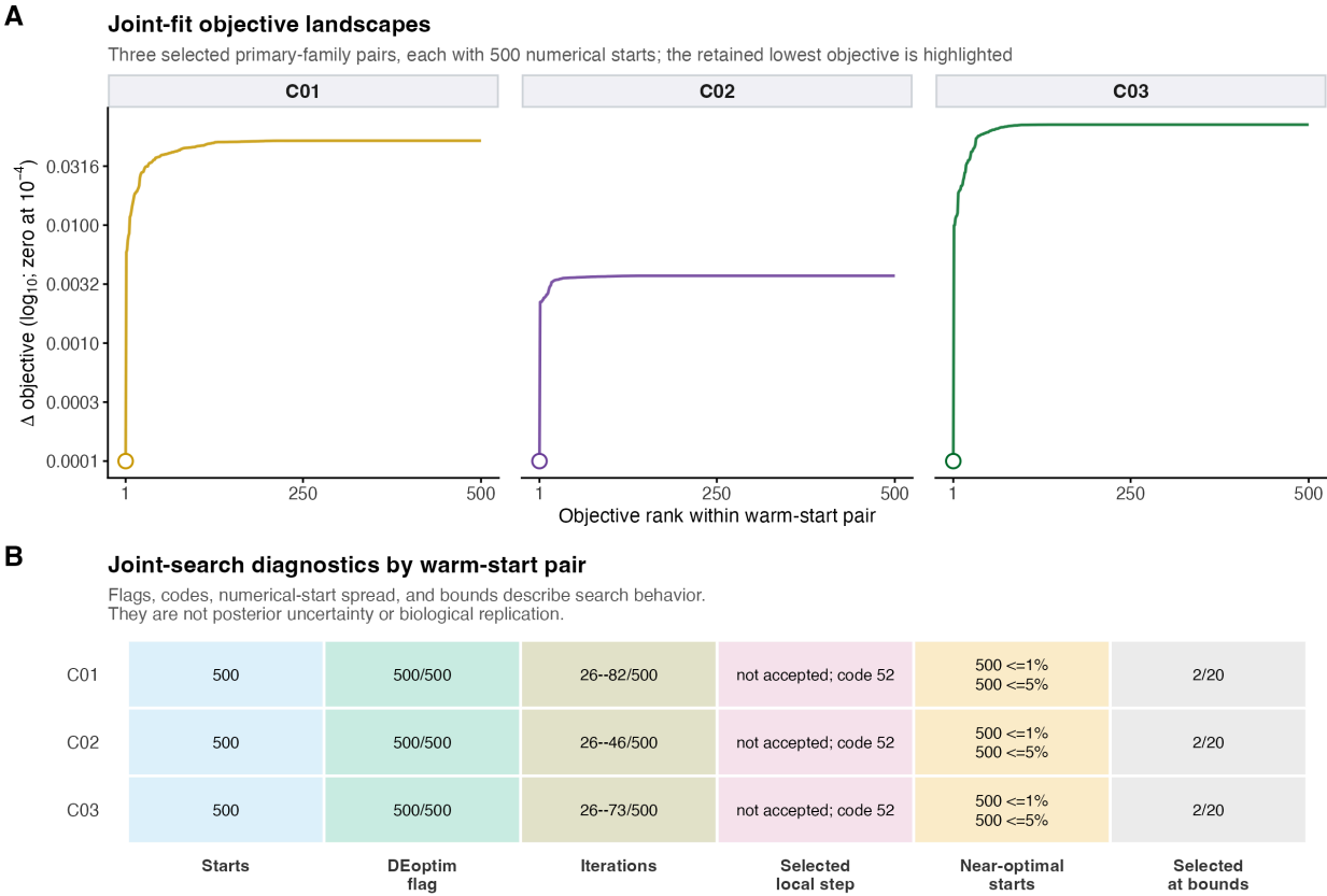
Supplementary Figure 4. Joint-fit numerical-search performance across the three retained primary-family pairs. (A) Objective-difference landscapes for the C01, C02, and C03 500-start joint fits. Within each retained pair, starts are ranked by objective, the lowest retained winner is highlighted, and exact zero is displayed at on the log axis. (B) Primary-family-resolved run diagnostics, including numbers of starts, recorded differential-evolution convergence flags, completed-iteration ranges relative to the target, selected local-step status and code, near-optimal start counts, and exact active-bound counts for the selected winners. The corresponding retained-pair rows are marked in Supplementary Table 7. These diagnostics characterize the sampled numerical searches; they are not biological replication, posterior distributions, confidence intervals, bootstrap uncertainty, profile likelihoods, held-out validation, or proof of a global optimum.
