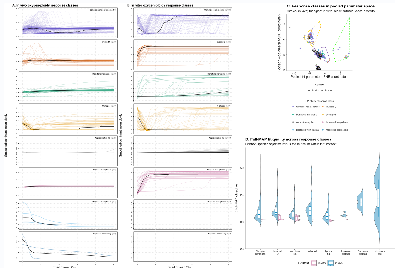
Supplementary Figure 5. {Separate-fit fixed-O response classes and their fitted-landscape context.} (A--B) Context-specific oxygen--ploidy response classes. Analytical dominant-eigenvector ploidy curves from the 500 separate in vivo fits (A) and 500 separate in vitro fits (B) were grouped by the same regression-smoothed response-shape rule. Both columns use the same fixed eight-class order; an empty plotting region therefore records a class absent from that context rather than omitted data. Class names and seed counts are printed in the upper-right corner. Thin colored curves show individual optimizer-seed endpoints and the black curve is the pointwise class median. Panel-specific ploidy ranges preserve visibility of both broad and nearly flat responses. These class counts include reliable, caution, and unreliable spectral-gap strata. (C) Response classes in pooled parameter space. All 1,000 separate-fit endpoints are positioned in the pooled 14-parameter t-SNE coordinate system used for the joint warm-start landscape in Figure 5C and colored by fixed-O response class. Circles denote in vivo and triangles denote in vitro . These unitless visualization coordinates have no direct mechanistic interpretation and are distinct from the in vivo -only 18-parameter embedding in Figure 4B. A black outline marks the lowest-objective endpoint within every nonempty context--class combination. Dashed outlines delimit the C01, C02, and C03 in vivo warm-start regions using the same gold, purple, and green colors as Figure 5; they are search-design regions rather than biological groups. (D) Context-relative full-MAP fit quality across response classes. For each context, the minimum full MAP objective across its 500 separate fits was subtracted before comparison. Blue left and pink right half-violins show the in vivo and in vitro distributions, respectively, with narrow context-colored boxplots showing medians and interquartile ranges. Empty halves identify classes absent from that context. Because the two fits use different observation models, this within-context objective difference is used only to compare relative fit quality among response classes; vertical values are not cross-context likelihood ratios. Class and reliability counts are reported in Supplementary Table 9. Together, panels C--D diagnose remaining fitted-landscape multiplicity rather than selecting one response shape a priori.
