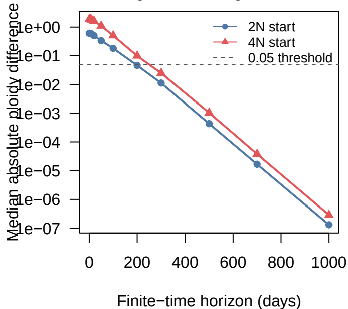
Convergence to eigen attractor
