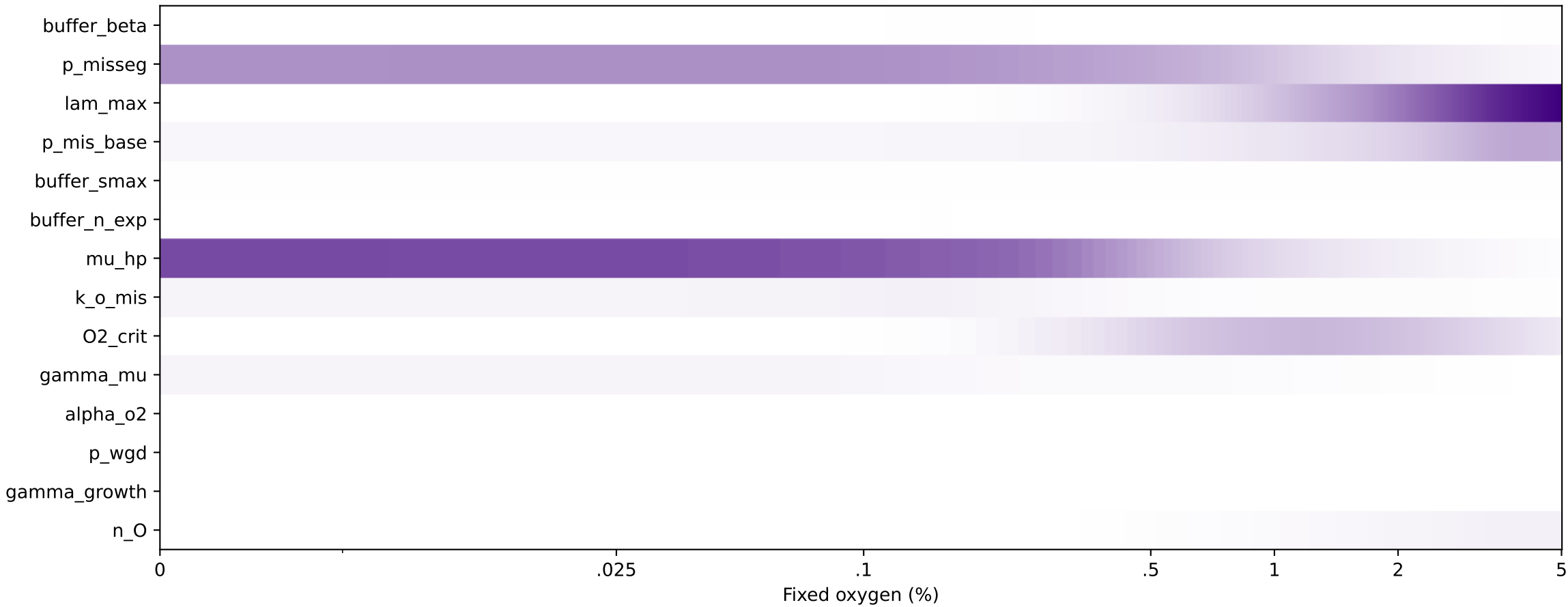
Asymptotic net live-cell growth rate | First-order effects (S1) | eFAST N=513, mean across replicates
