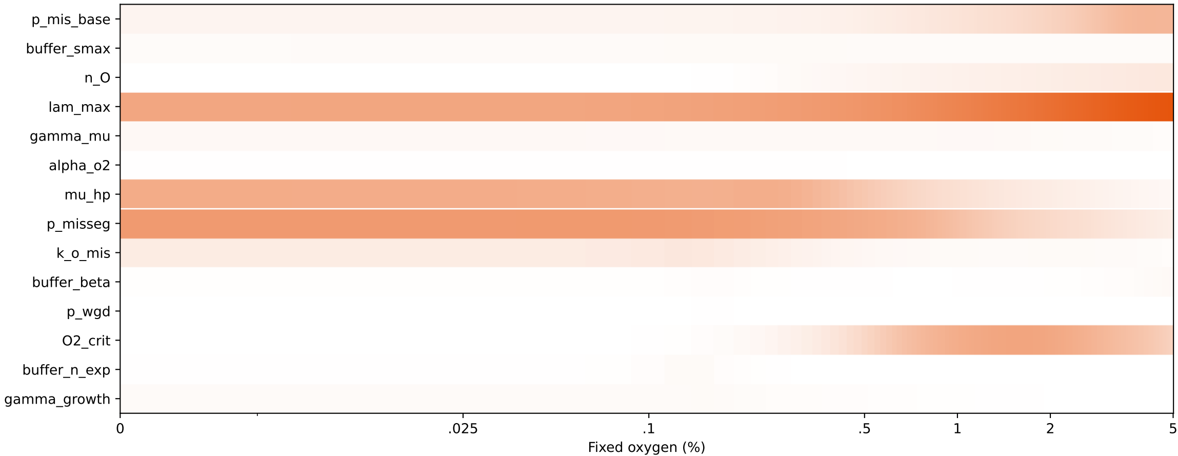
Asymptotic net live-cell growth rate | Total effects (ST) | eFAST N=513, mean across replicates
