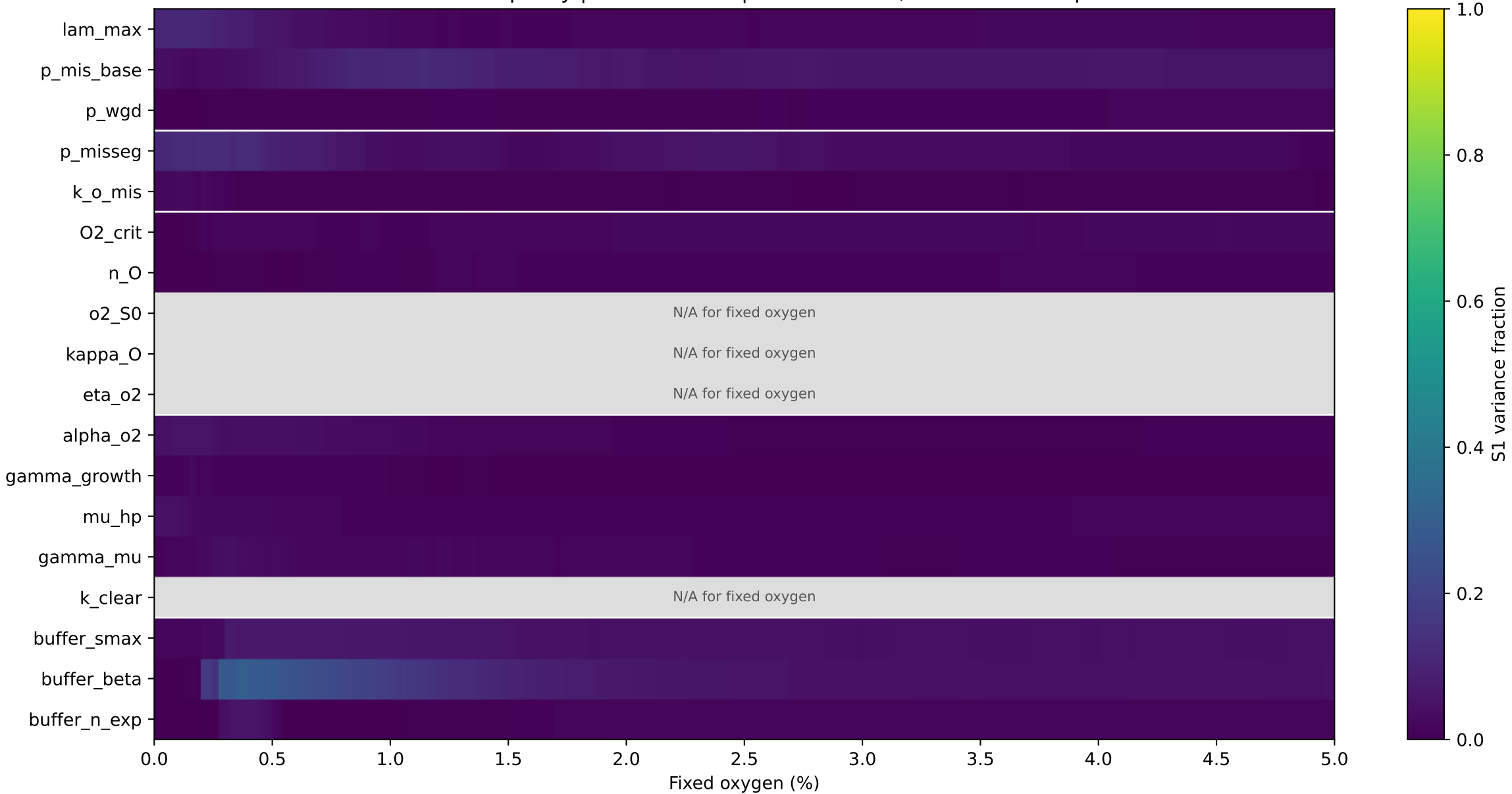
Dominant mean ploidy | First order S1 | eFAST N=513, mean across replicates
