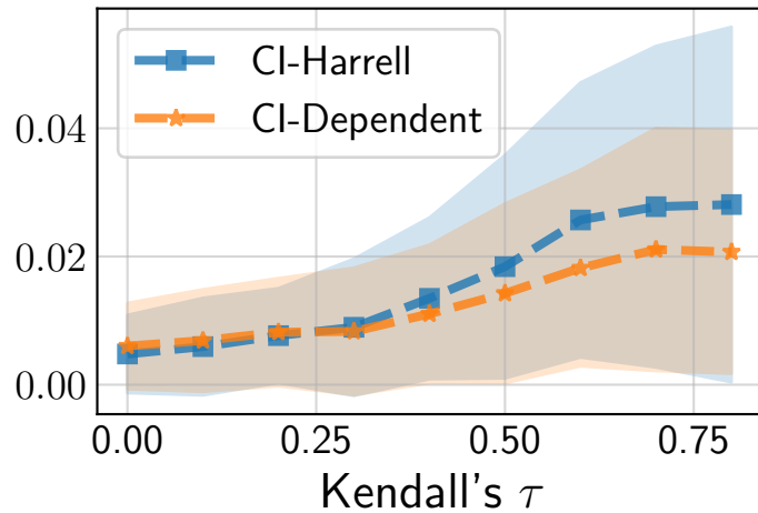
Frank Copula
