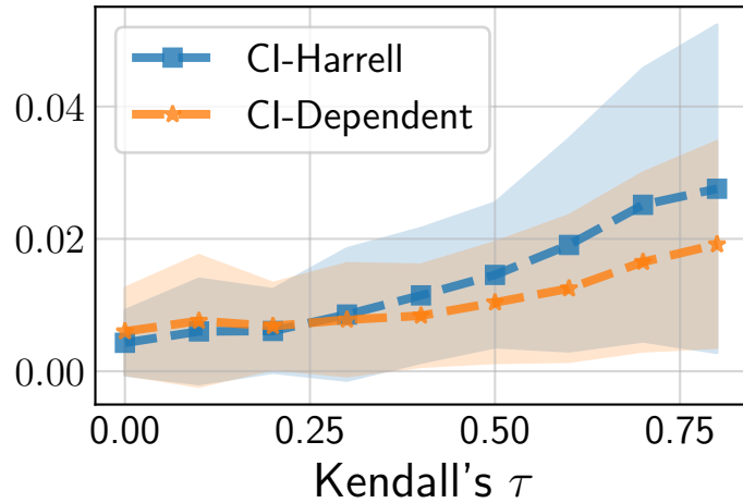
Clayton Copula
