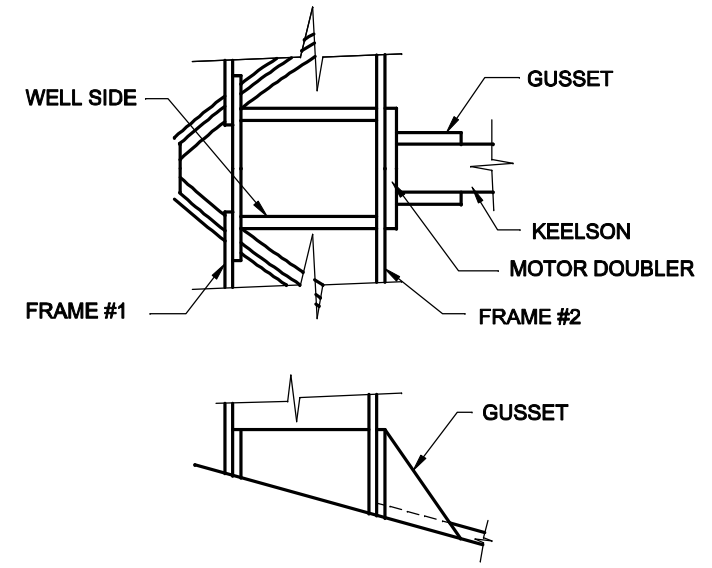
OUTBOARD WELL DETAILS
