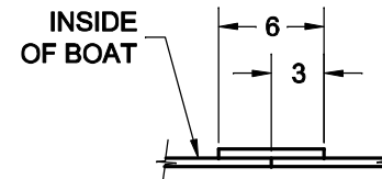
BUTT BLOCK DETAIL FOR ALL PLYWOOD SEAMS SCALE 2" = 1"
