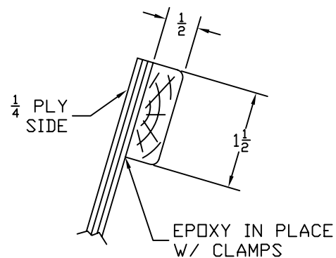
RUB RAIL DETAIL SCALE: FULL
