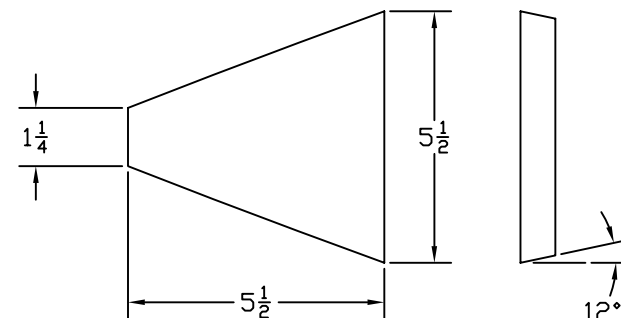
BREAST HOOK MAKE FROM 1X6 CLEAR FIR SCALE: 1/2
