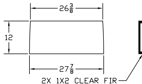
SEAT DETAIL MAKE FROM 1/2 ACX PLY SCALE: 1/10
