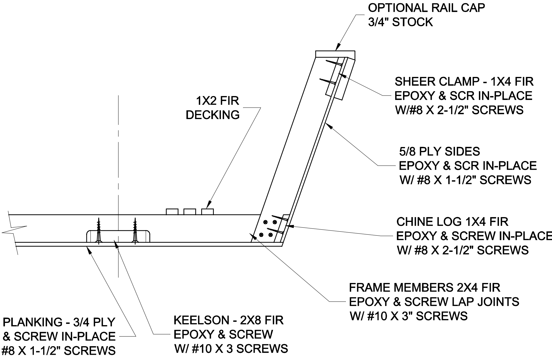
TYPICAL CONSTRUCTION METHOD ALL FRAME STATIONS SCALE 2" = 1'
