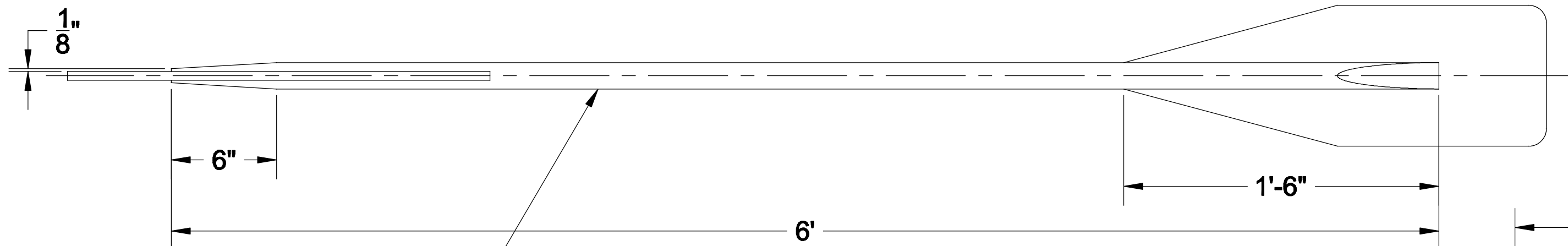
PADDLE ASSEMBLY
