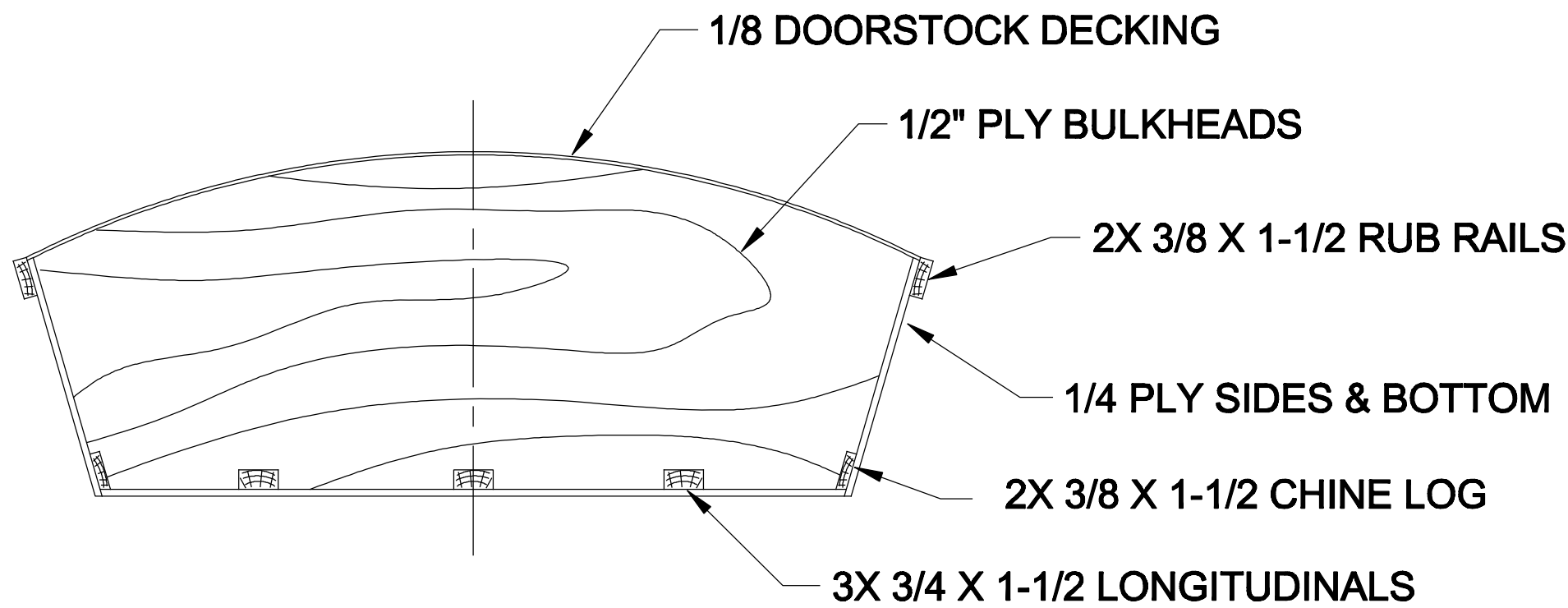
CONSTRUCTION DETAILS
