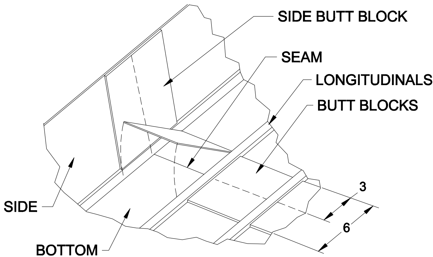
BUTT BLOCK PLACEMENT (VIEW FROM INSIDE OF BOAT)
