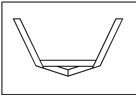
CUT OUT DECK BEAM, LOCATE IN POSITION, EPOXY & SCREW IN PLACE
