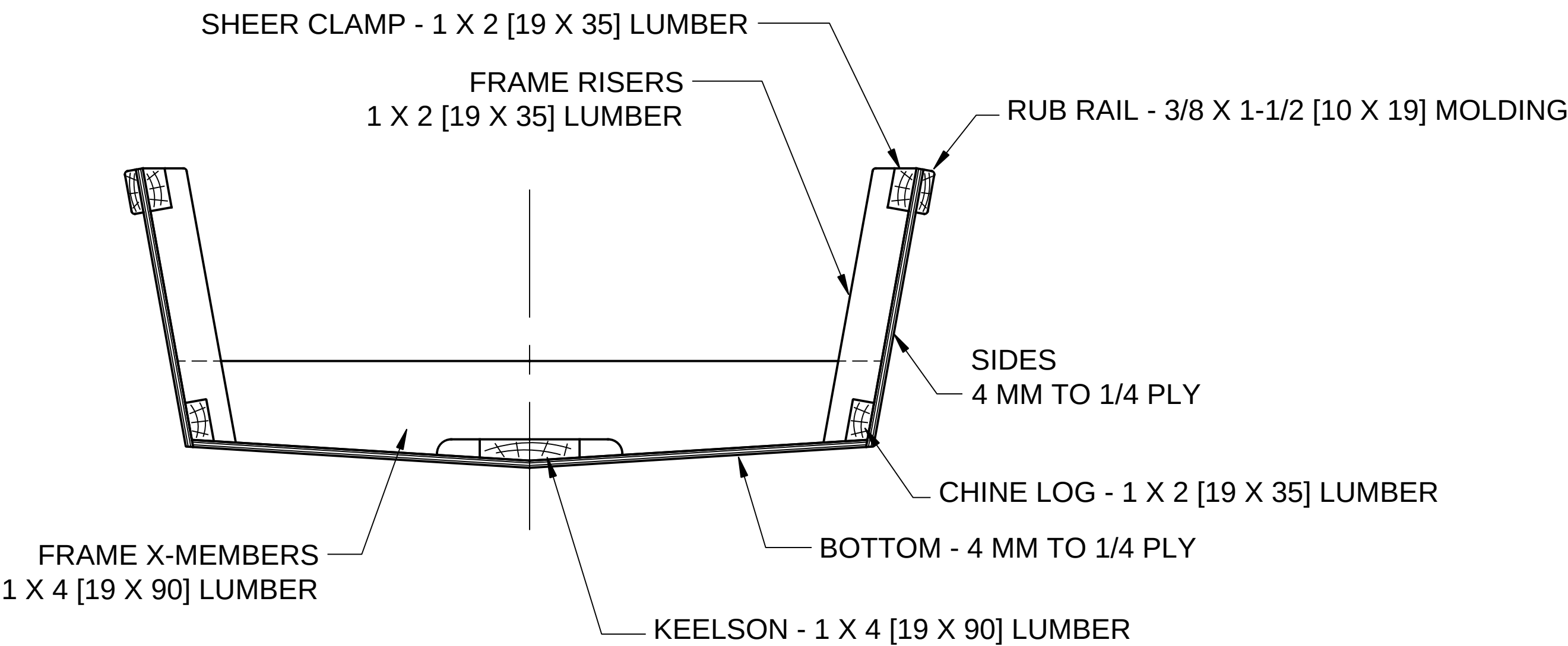
CROSS SECTION TYPICAL
