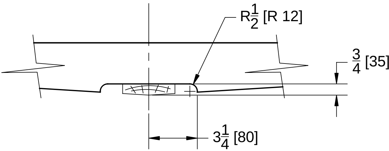
KEELSON CUTOUT TYPICAL - ALL FRAMES
