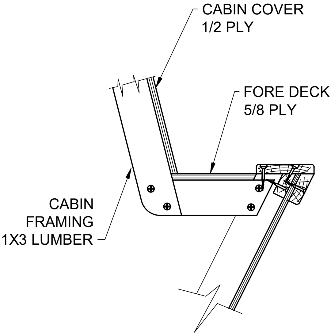
CONSTRUCTION DETAIL CABIN SECTION NOT TO SCALE
