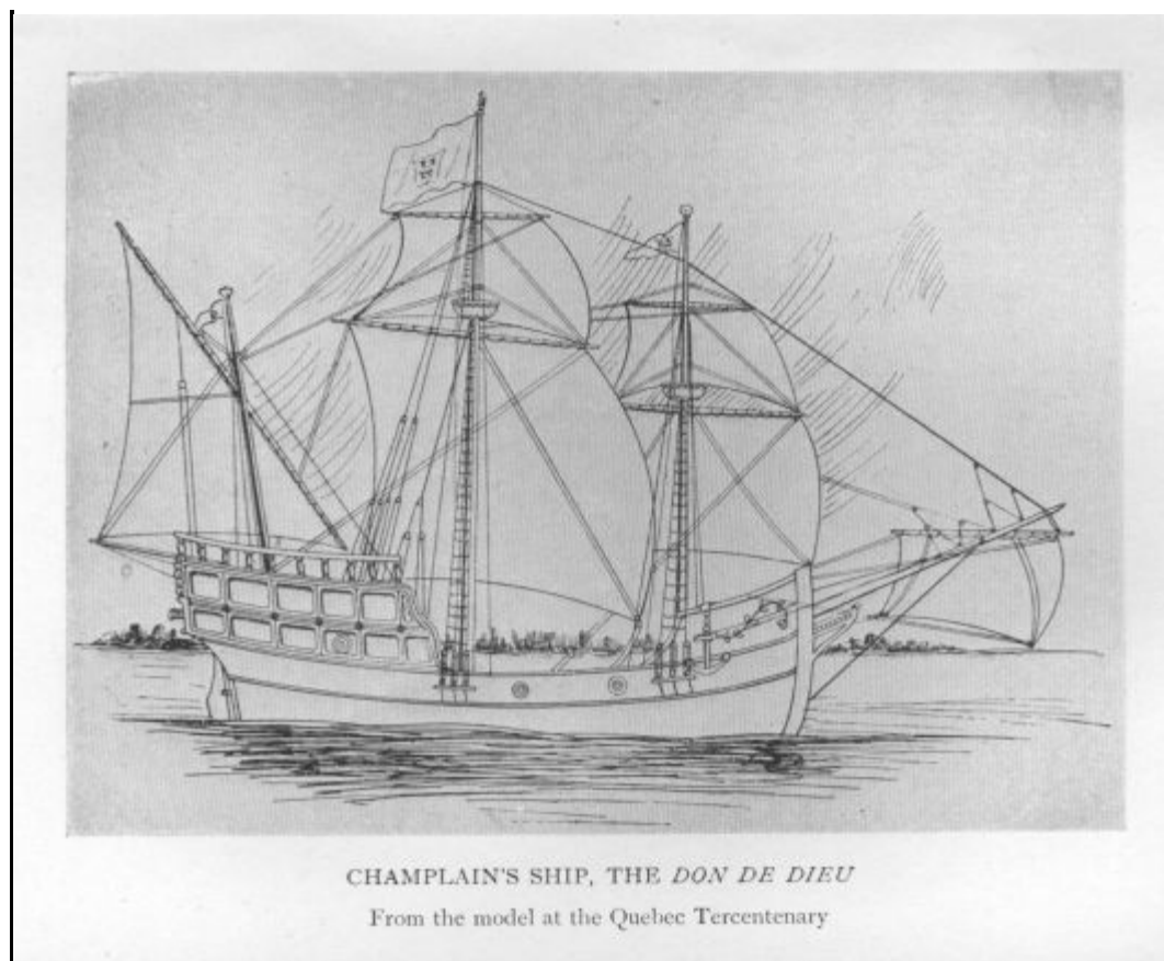
CHAMPLAIN'S SHIP, THE DON DE DIEU From the model at the Quebec Tercentenary
