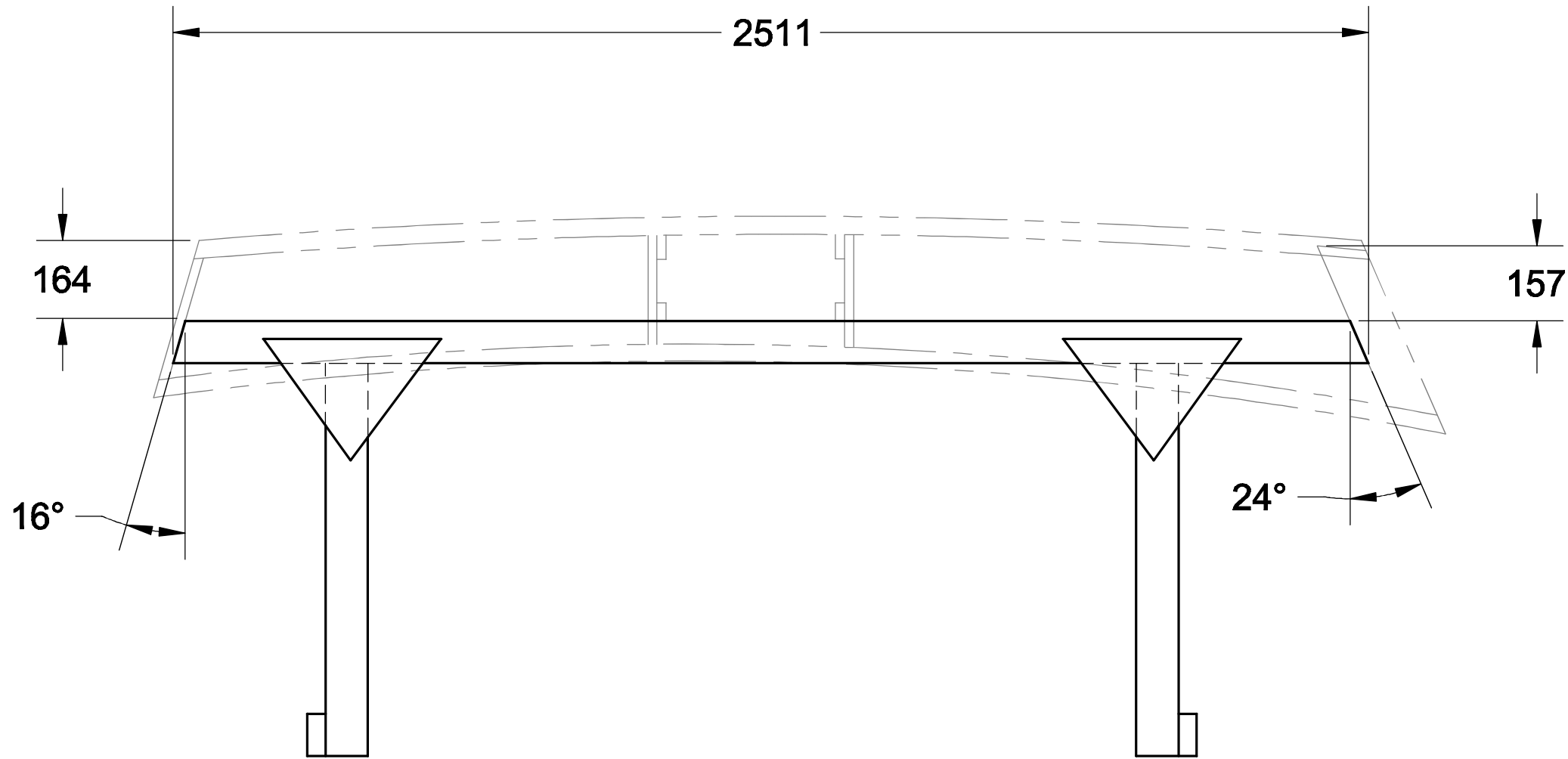
STRONGBACK JIG MAKE FROM SCRAP 35 X 90 TIMBER AND 10MM PLY
