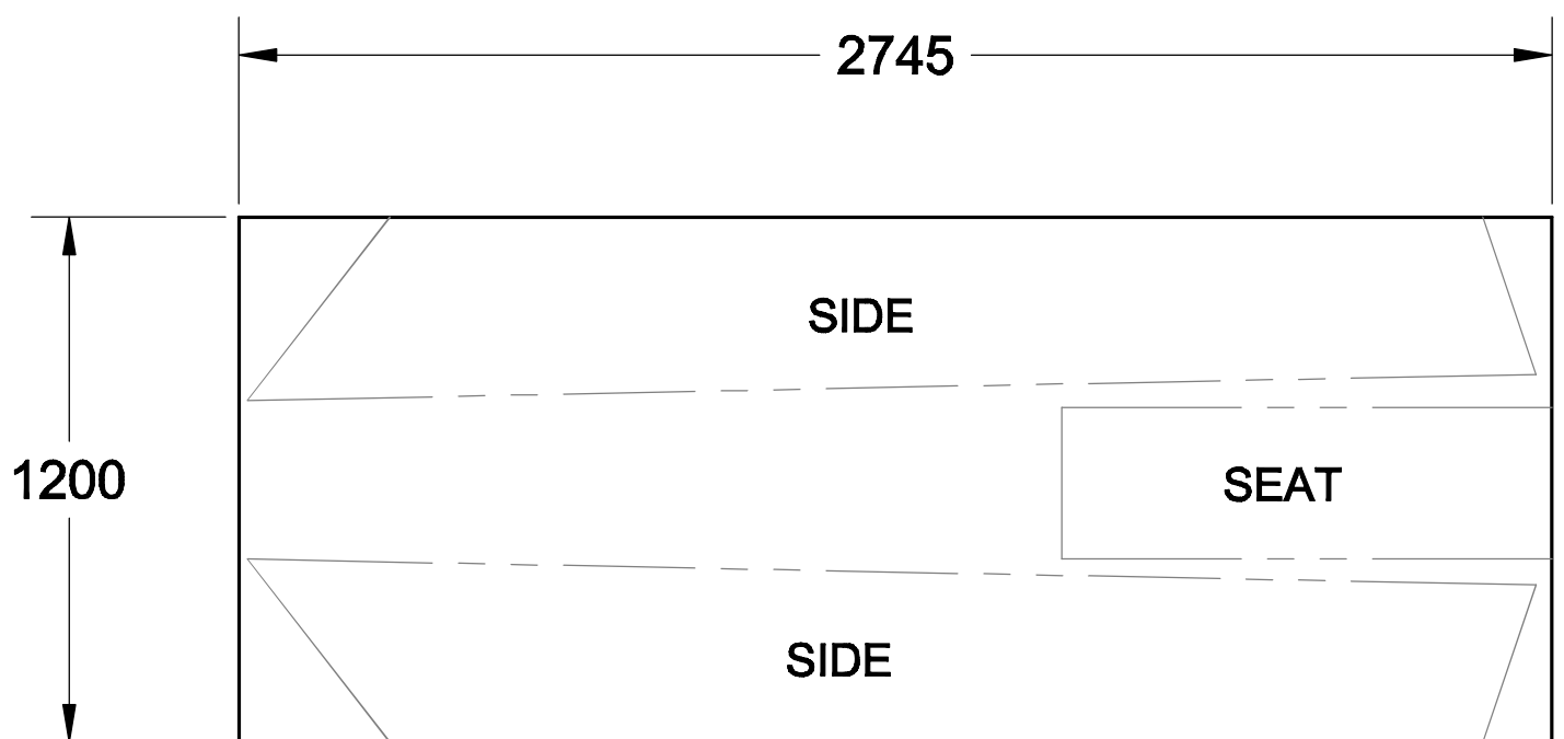
METHOD TO CUT OUT PANELS FROM 1 SHEET OF 1200 X 2745 PLY & 1 SHEET OF 1200 X 2400 PLY NO SCALE
