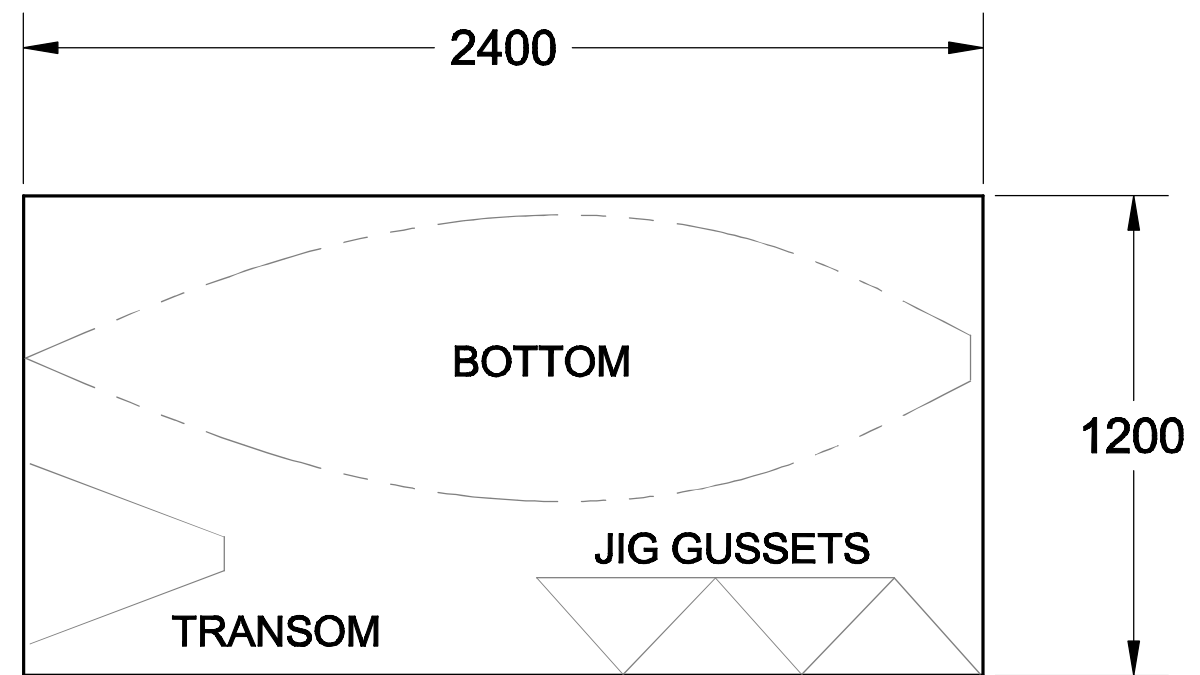
METHOD TO CUT OUT PANELS FROM 1 SHEET OF 1200 X 2745 PLY & 1 SHEET OF 1200 X 2400 PLY NO SCALE
