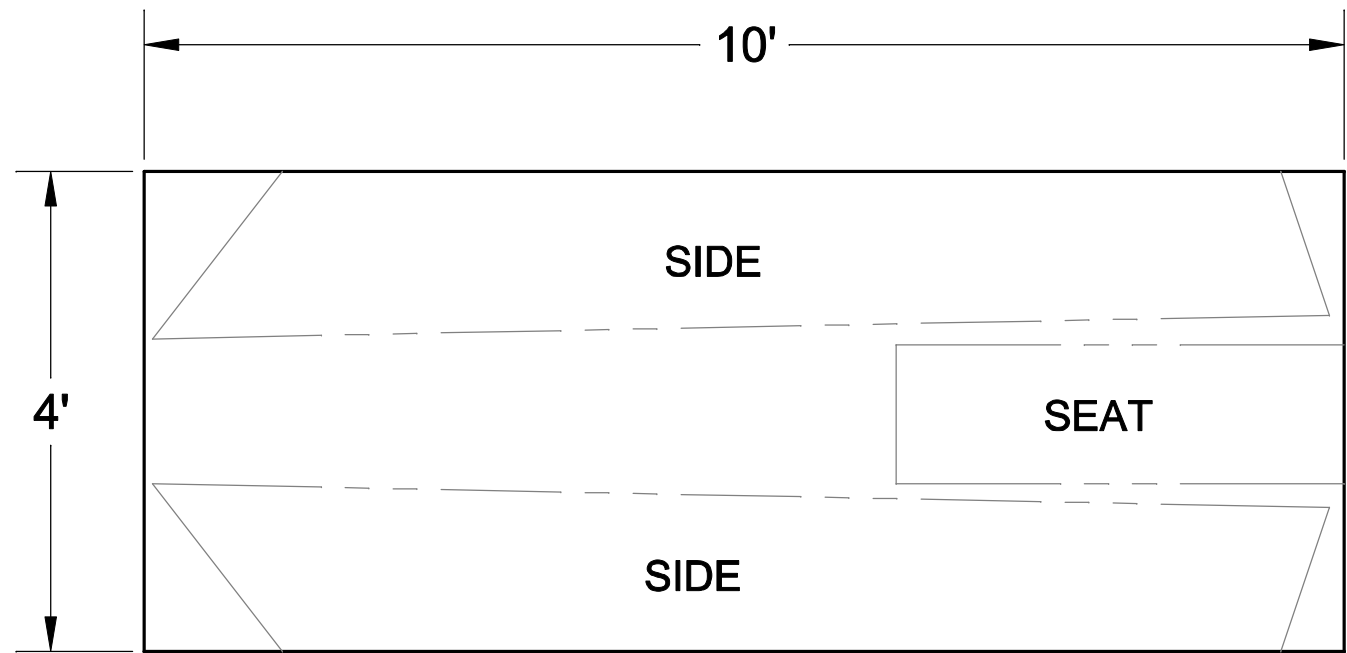
METHOD TO CUT OUT PANELS FROM 1 SHEET OF 4' X 10' PLY & 1 SHEET OF 4' X 8' PLY NO SCALE
