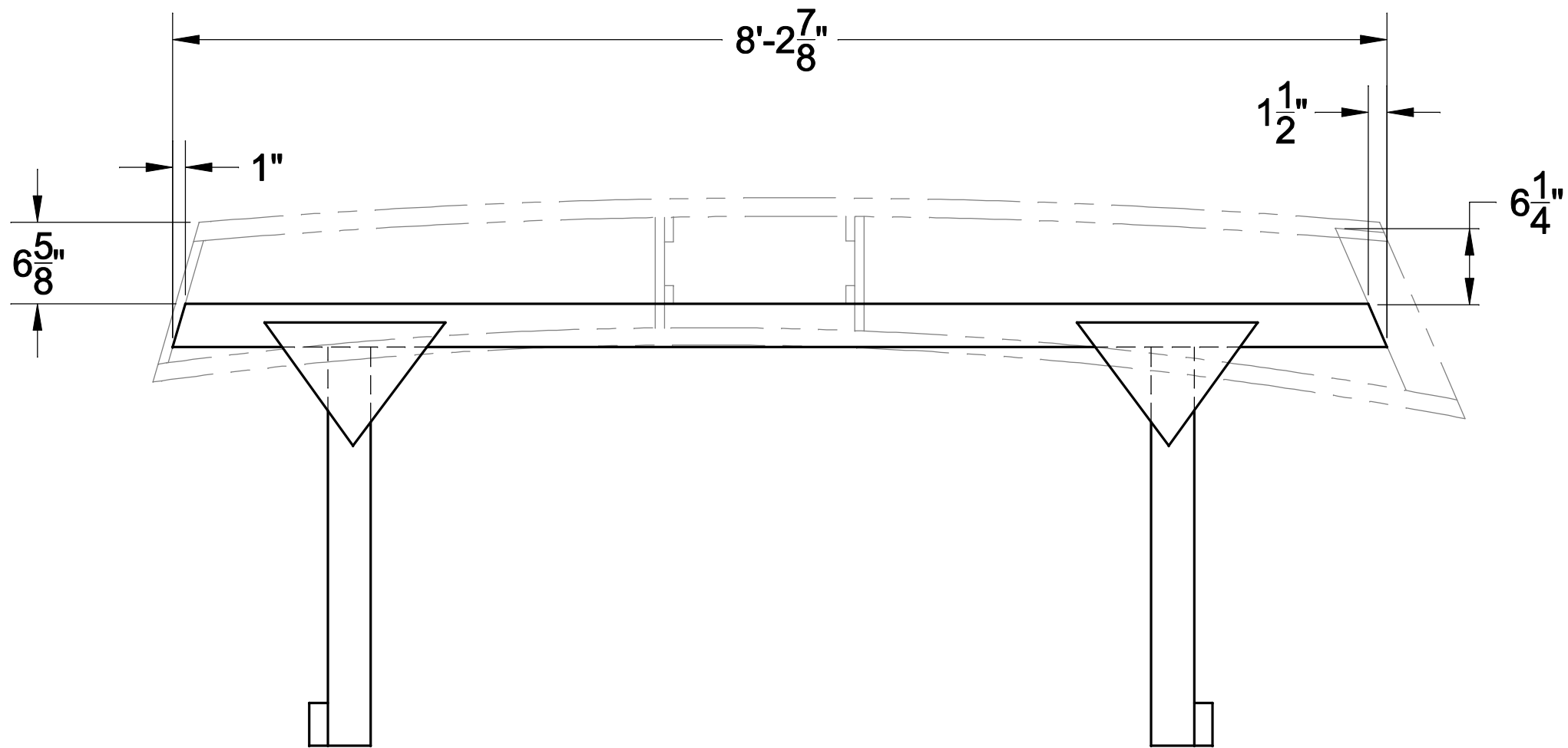
STRONGBACK JIG MAKE FROM SCRAP 2X4S AND 3/8" PLY
