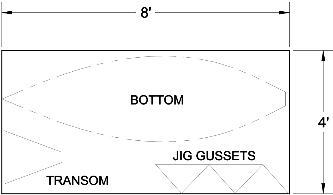
METHOD TO CUT OUT PANELS FROM 1 SHEET OF 4' X 10' PLY & 1 SHEET OF 4' X 8' PLY NO SCALE
