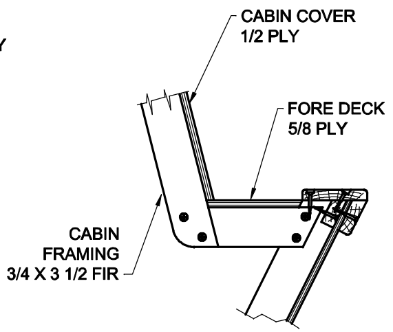
FORWARD SECTIONS CABIN CONSTRUCTION NO SCALE
