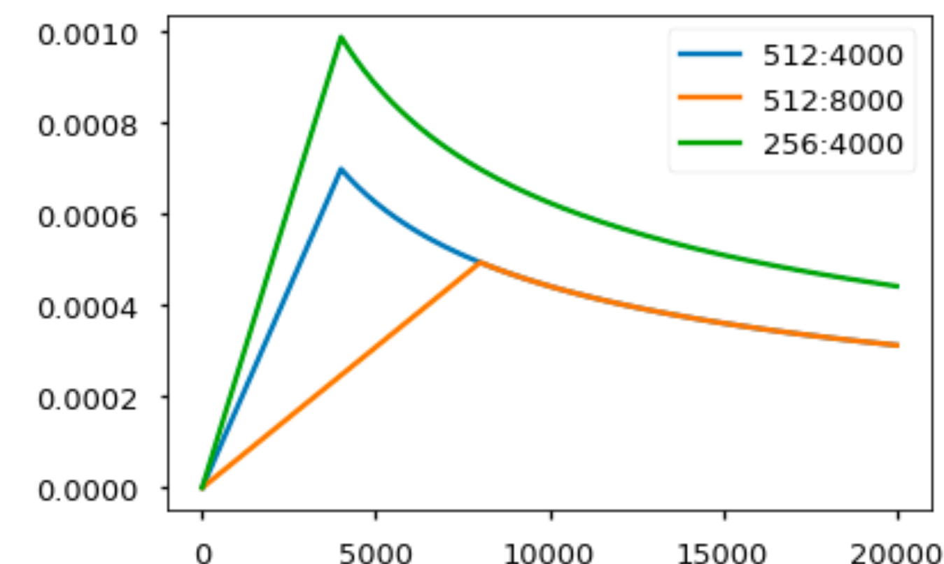
lr schedule
