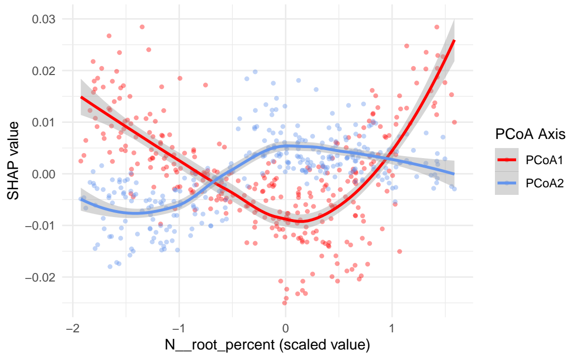
SHAP Values vs Scaled N__root_percent
