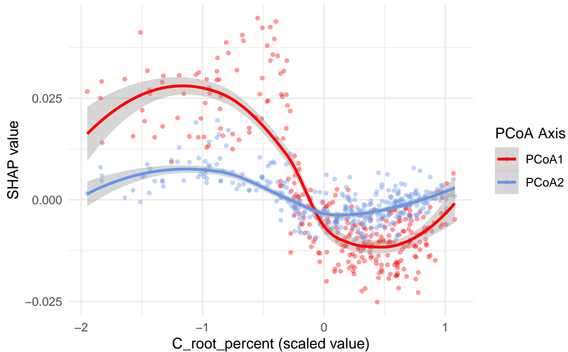
SHAP Values vs Scaled C_root_percent
