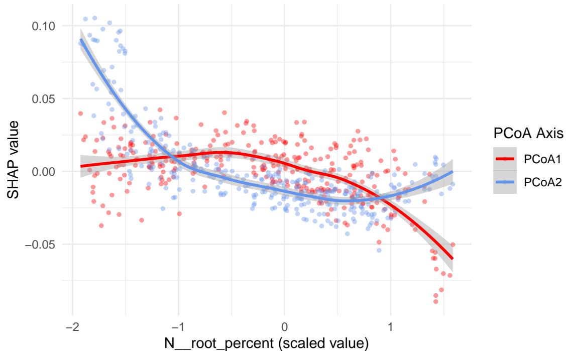
SHAP Values vs Scaled N__root_percent (Fungi)
