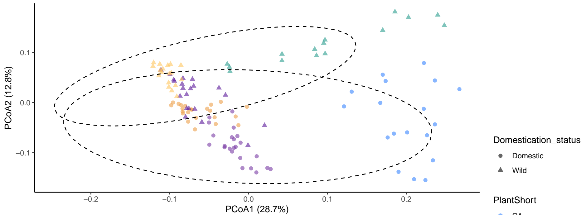
Fungi Wild vs Domestic PCoA
