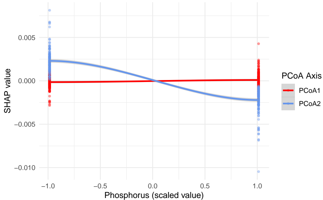
SHAP Values vs Scaled Phosphorus
