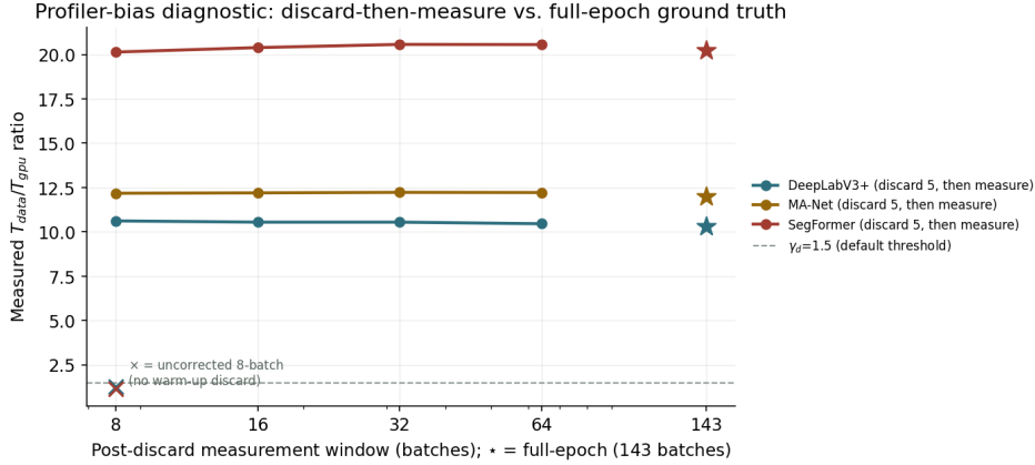
Figure 6: Measured ratio by post-discard window size against the full-epoch ground truth, all three architectures. The \times markers are the uncorrected 8-batch measurement (no discard) for comparison.
