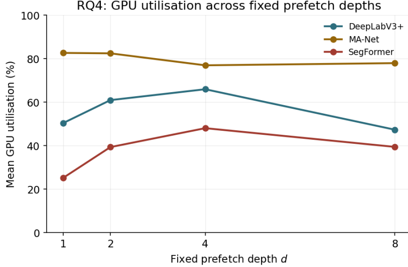
Figure 5: GPU utilisation across the fixed prefetch-depth sweep, all three architectures. DeepLabV3+ and SegFormer both peak at d = 4 ; MA-Net is flat.
