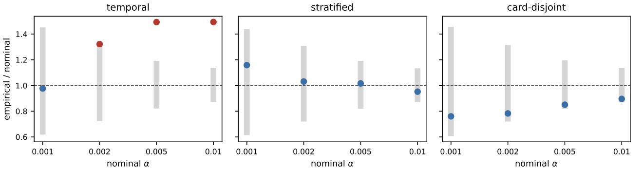
Figure 1: The same data as Table ??, with the Beta-Binomial interval drawn to scale. The interval widens sharply as \alpha tightens, which is why the temporal arm’s apparent compliance at \alpha = 0.001 is weak evidence rather than a pass: at that level the law admits almost anything.
