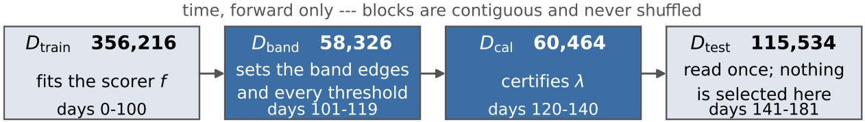
Figure 1: The four-block temporal split; shaded blocks carry the guarantee. Counts and day ranges are read from splits.csv , not typed.
