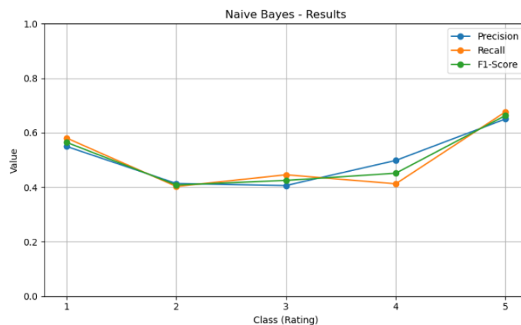
Abbildung 6.: Classification Report, Naive Bayes
