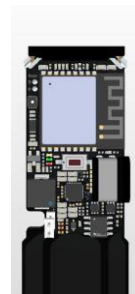
Left to right — rendered in singular plant use: solar harvesting, no wiring, no scheduled maintenance · v1.2 board in hand, beside its CAD model; prototype batch of 10, fully hardware validated · board in enclosure · PCB top view of the electronics region, 22 × 42 mm.
