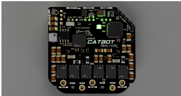
FlexNode v1.0 — STM32G4, DRV8353S and the six-FET power stage.
