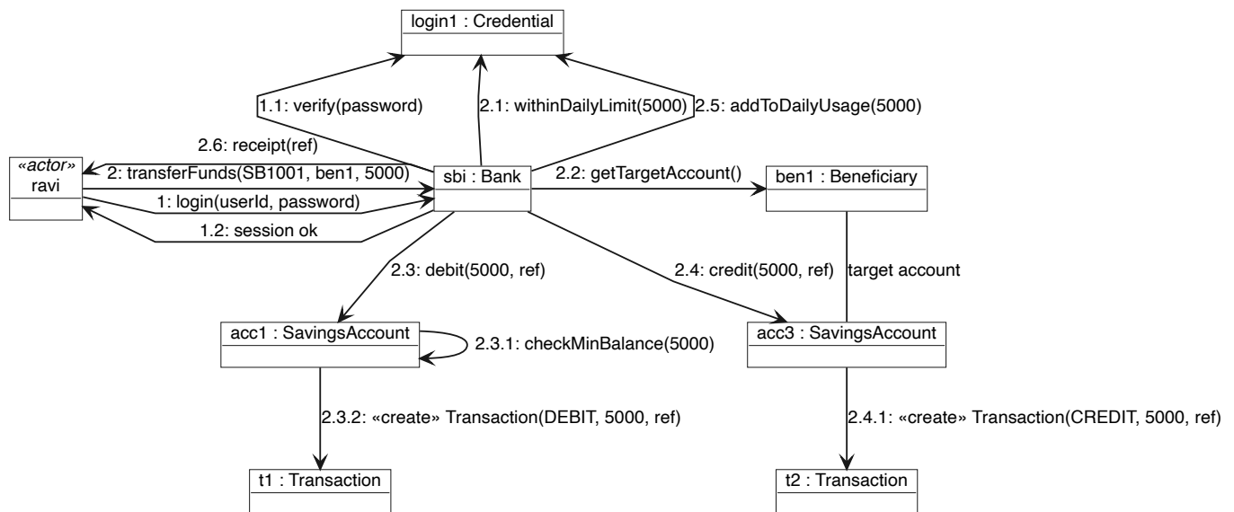
Collaboration Diagram - Online Banking System (Transfer Funds)
