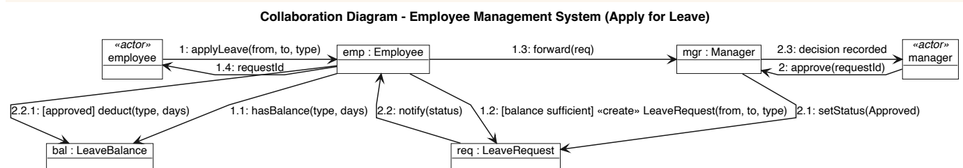
Collaboration Diagram - Employee Management System (Apply for Leave)
