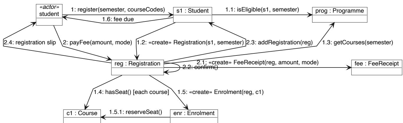
Collaboration Diagram - Student Registration (Register for Semester)
