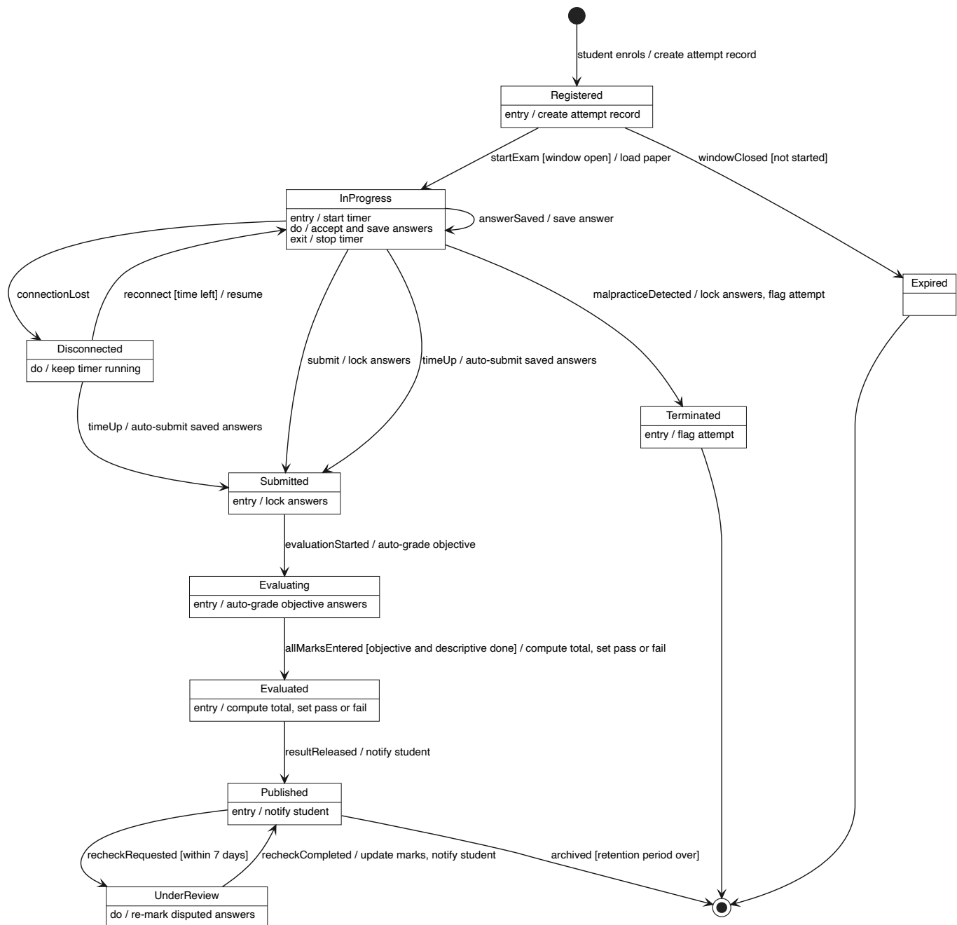
State Chart: ExamAttempt (Online Examination System)
