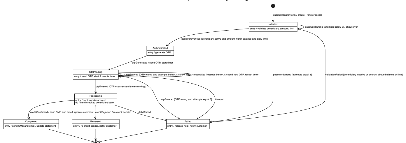
State Chart: Transfer (Online Fund Transfer through Net Banking)
