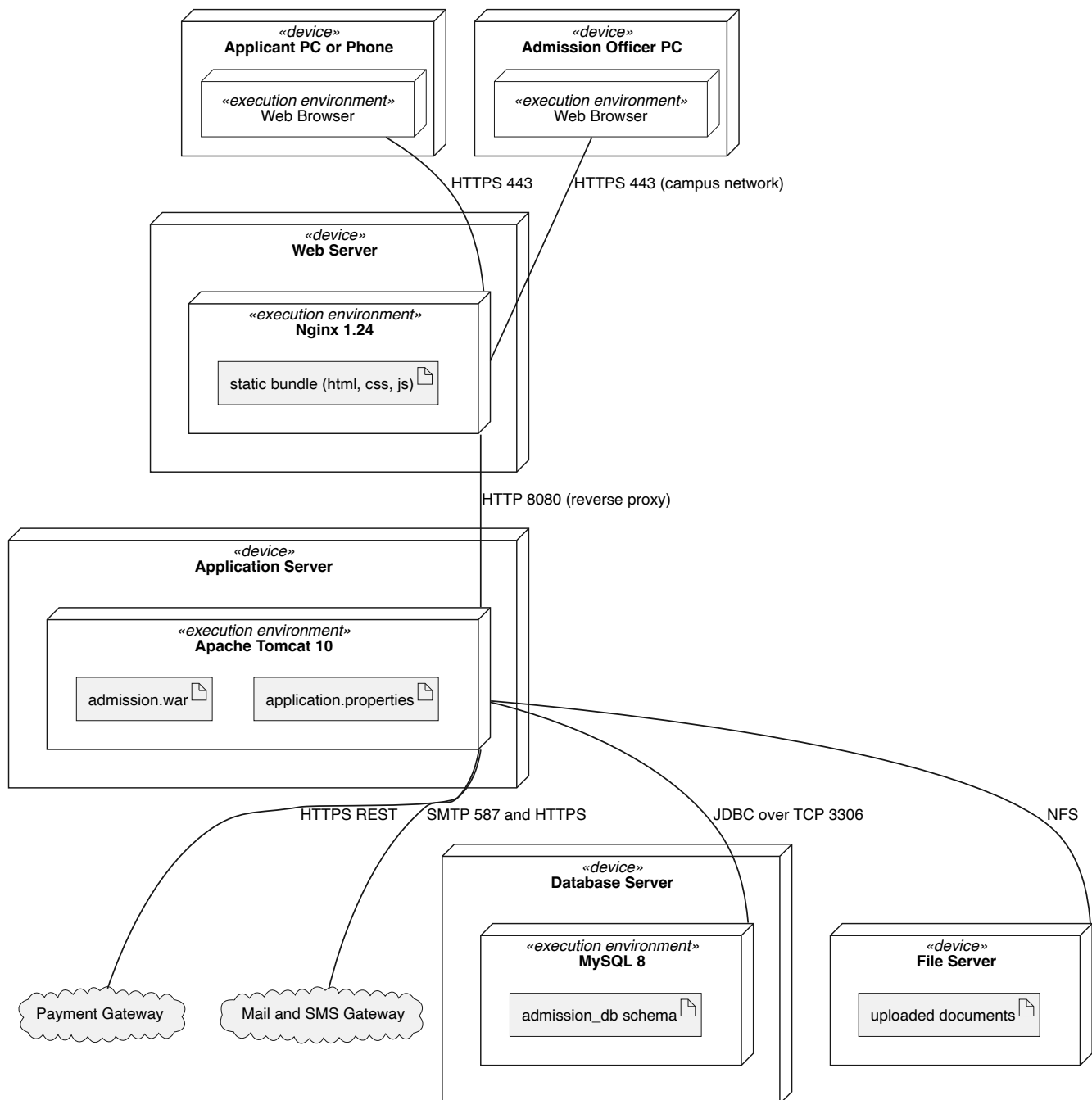
Deployment Diagram: Online Student Admission System
