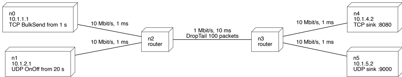
Topology: dumbbell, TCP and UDP sharing a 1 Mbit/s bottleneck
