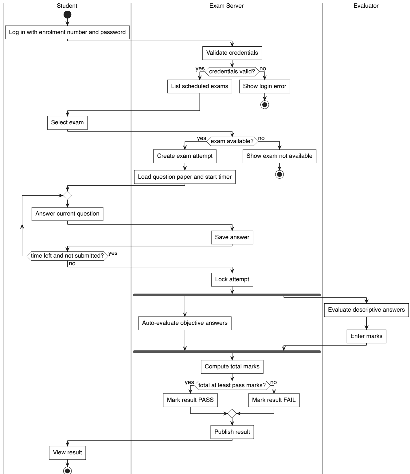
Activity Diagram: Online Examination System
