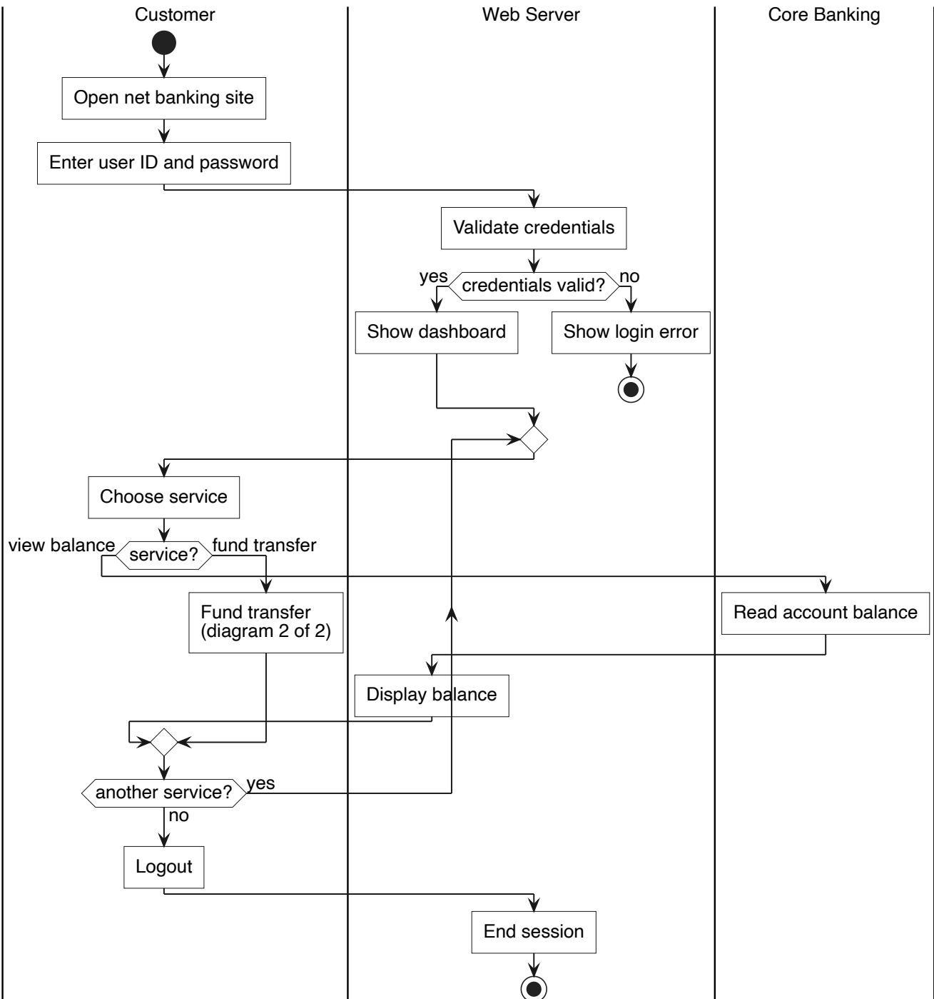
Activity Diagram: Online Banking System, part 1 of 2: login and service menu
