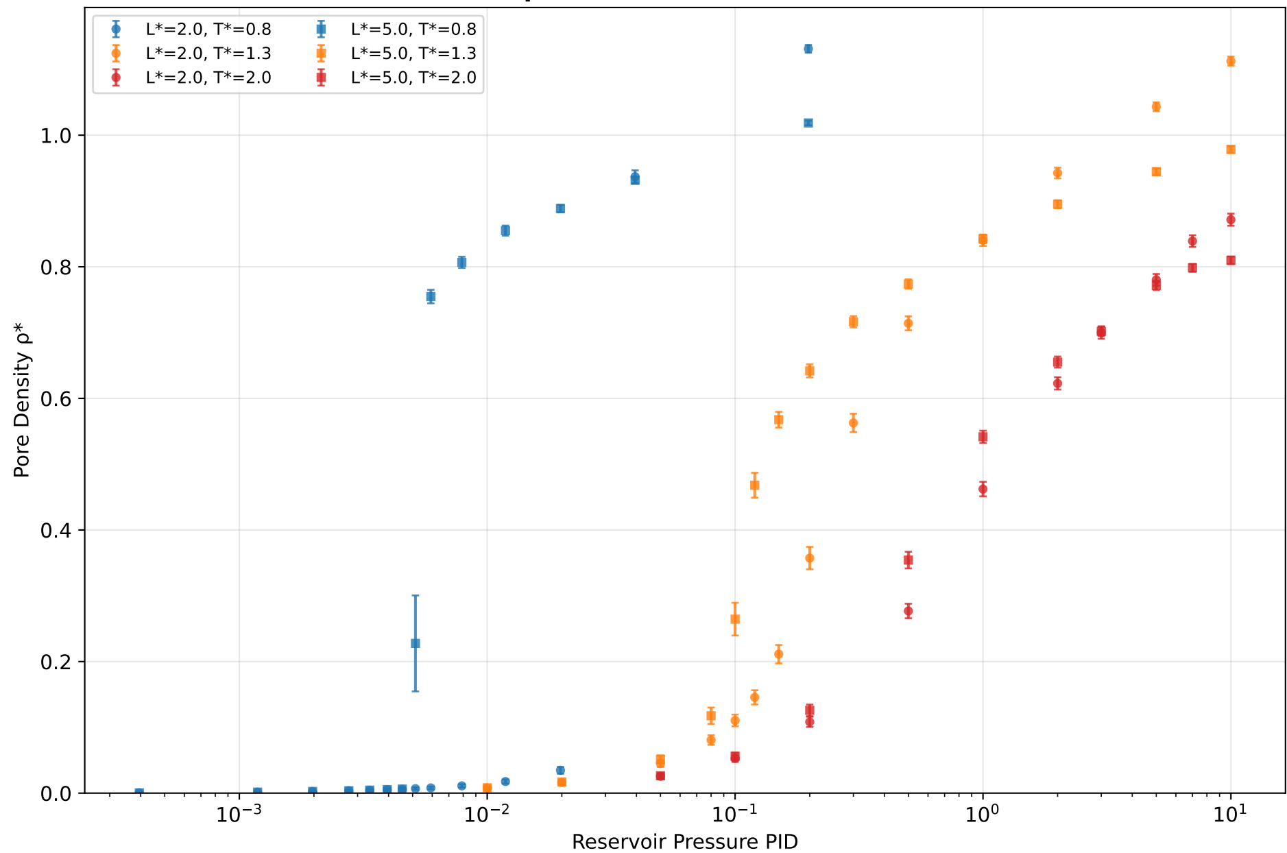
Complete Dataset: All Isotherms
