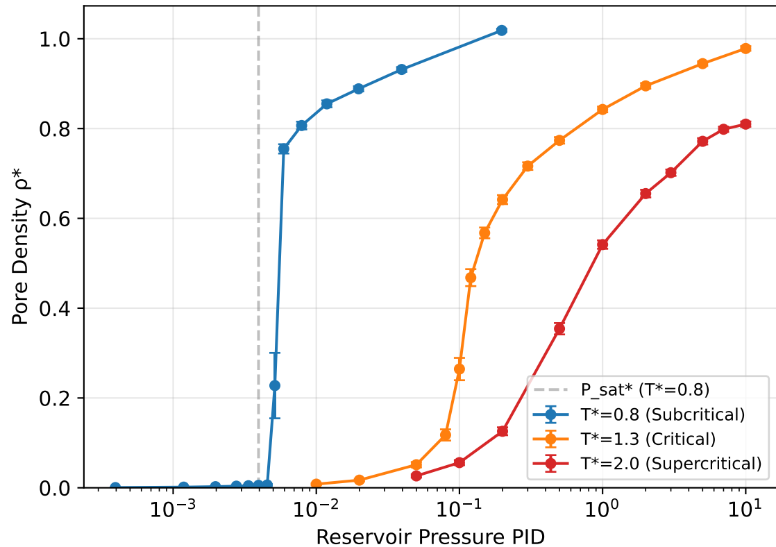
Slit Pore L^* = 5.0\sigma
