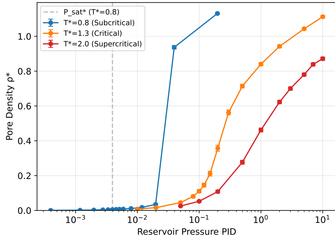
Slit Pore L^* = 2.0\sigma
