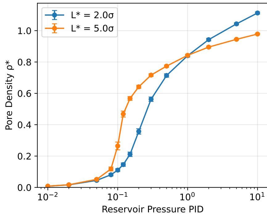
T^* = 1.3 (Critical)
