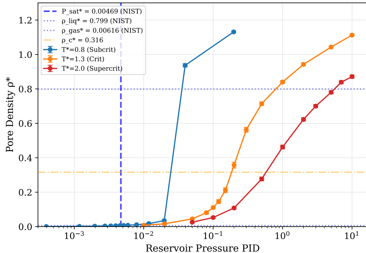
Slit Pore L^* = 2.0\sigma
