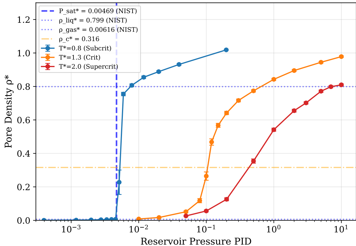
Slit Pore L^* = 5.0\sigma
