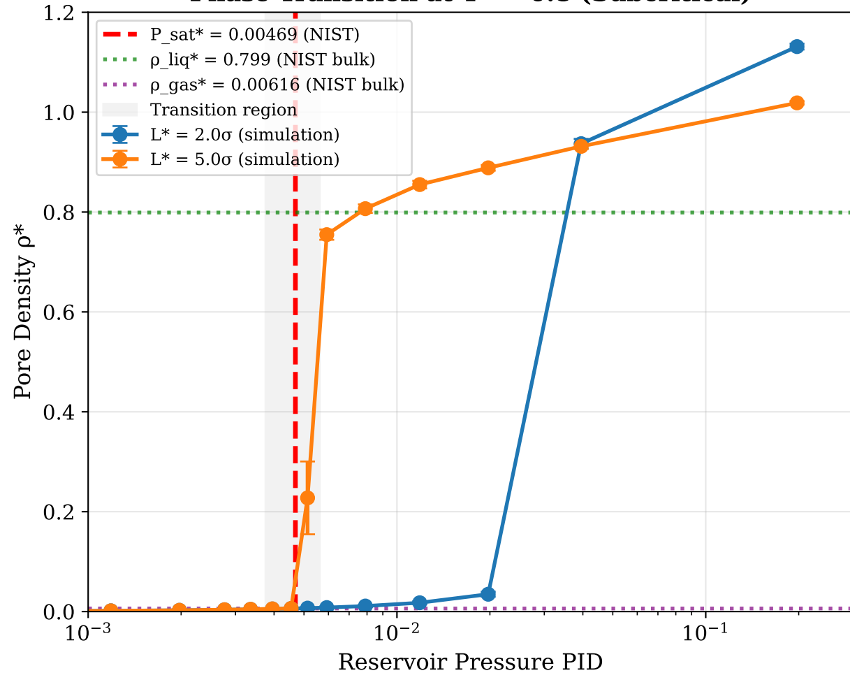
Phase Transition at T^* = 0.8 (Subcritical)
