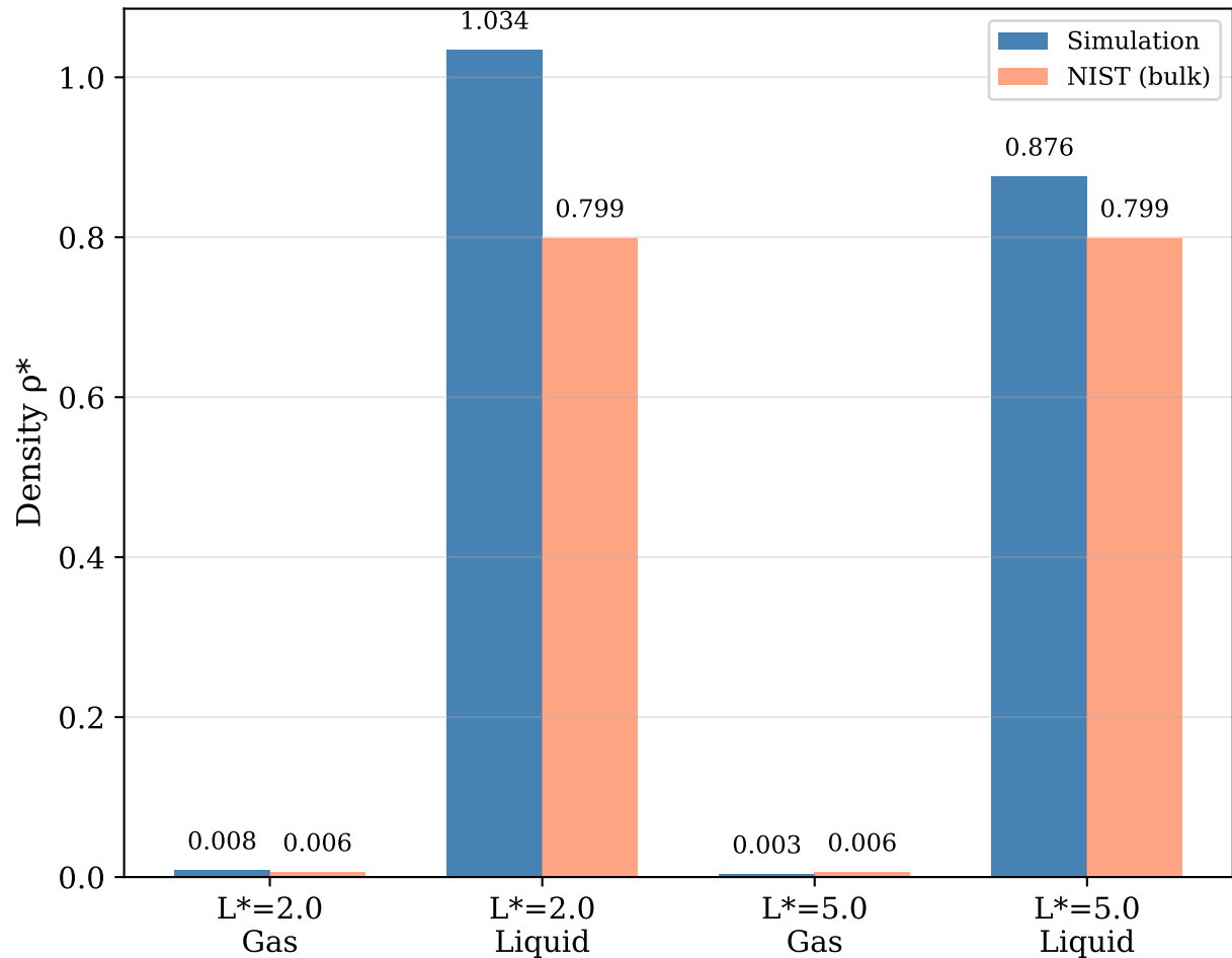
Simulation vs NIST Reference ( T^* = 0.8 )
