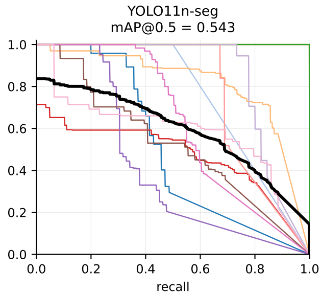
Mask precision-recall (IoU 0.5), test split
