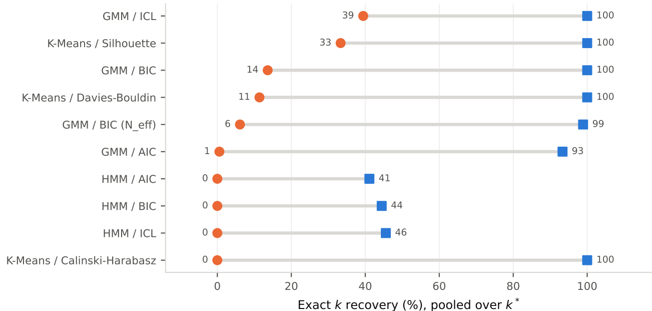
(a) Identical code, identical candidate range, 90 series each: only the data differs
