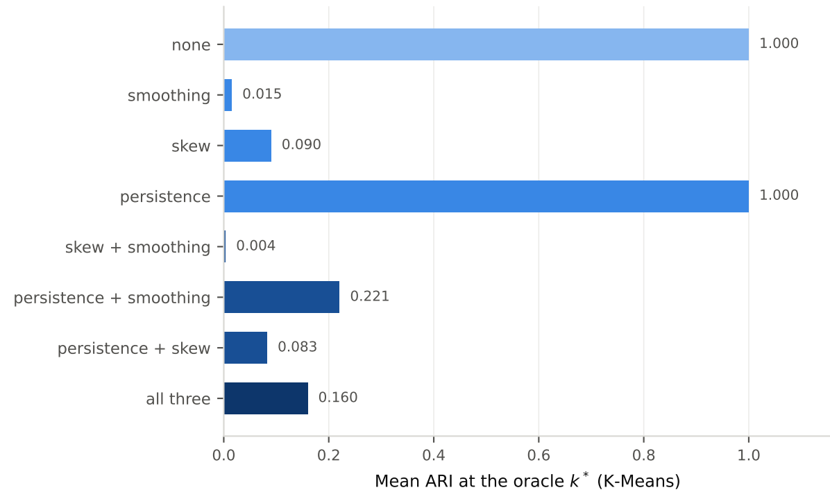
(a) How much structure survives in the feature
