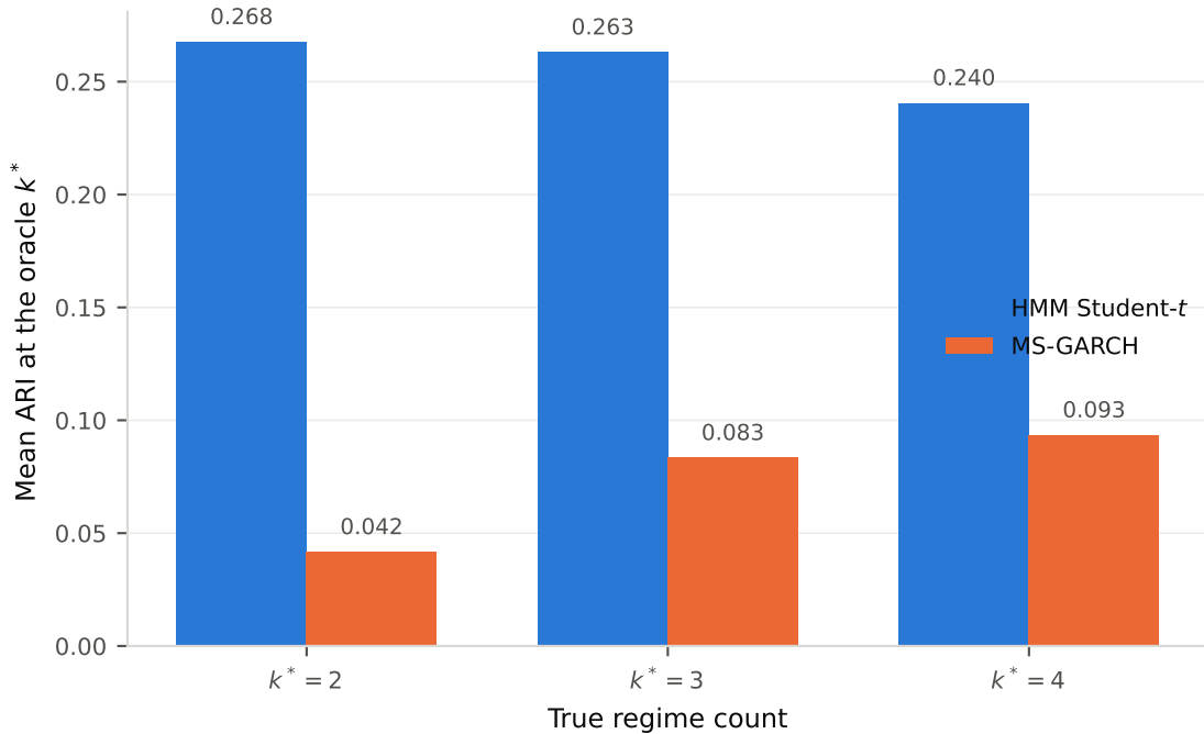
Partition quality at the oracle k^* by generative family
