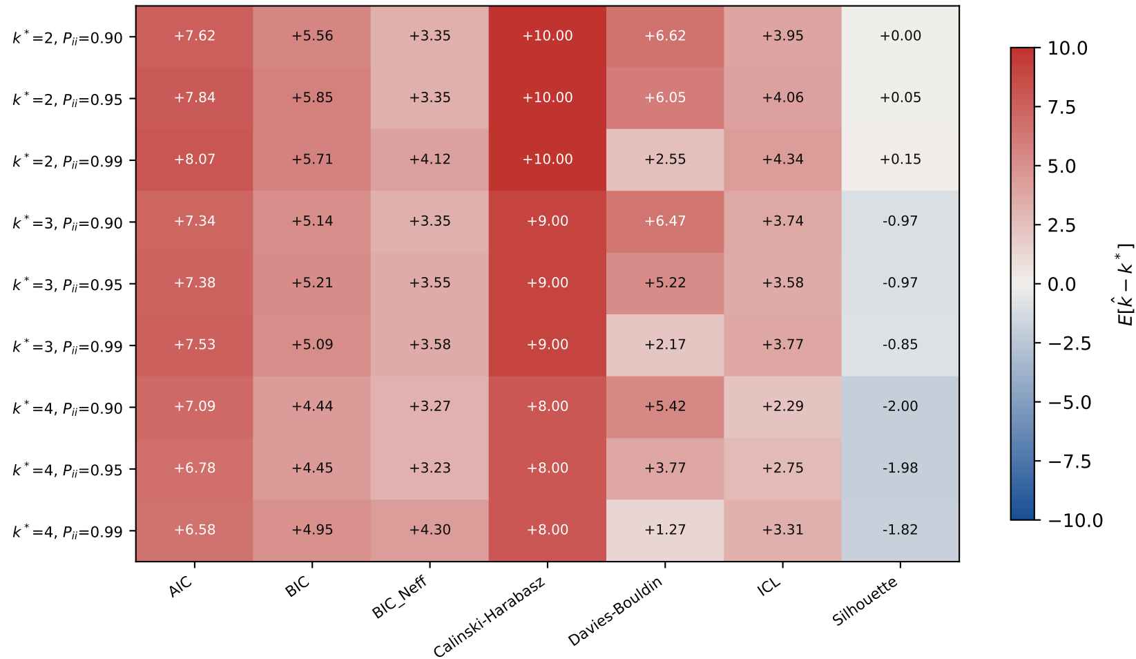
Signed bias E[\hat{k} - k^*] by true k^* and persistence
