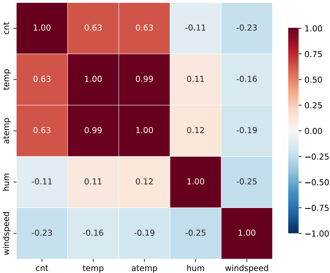
Pairwise correlations
