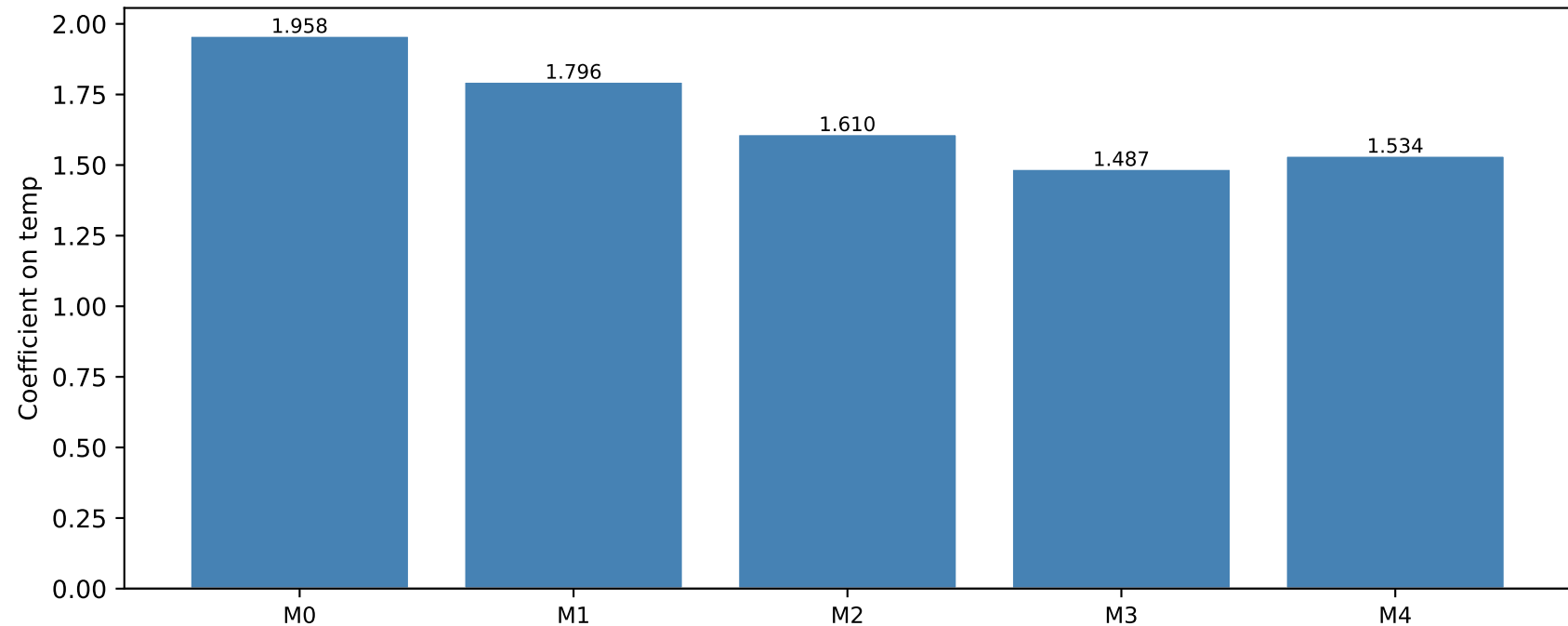
OVb demonstration: temp coefficient shrinks as confounders are added
