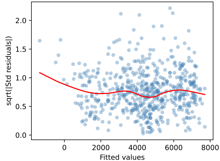
Scale-Location
