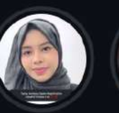
QnA Competi...
