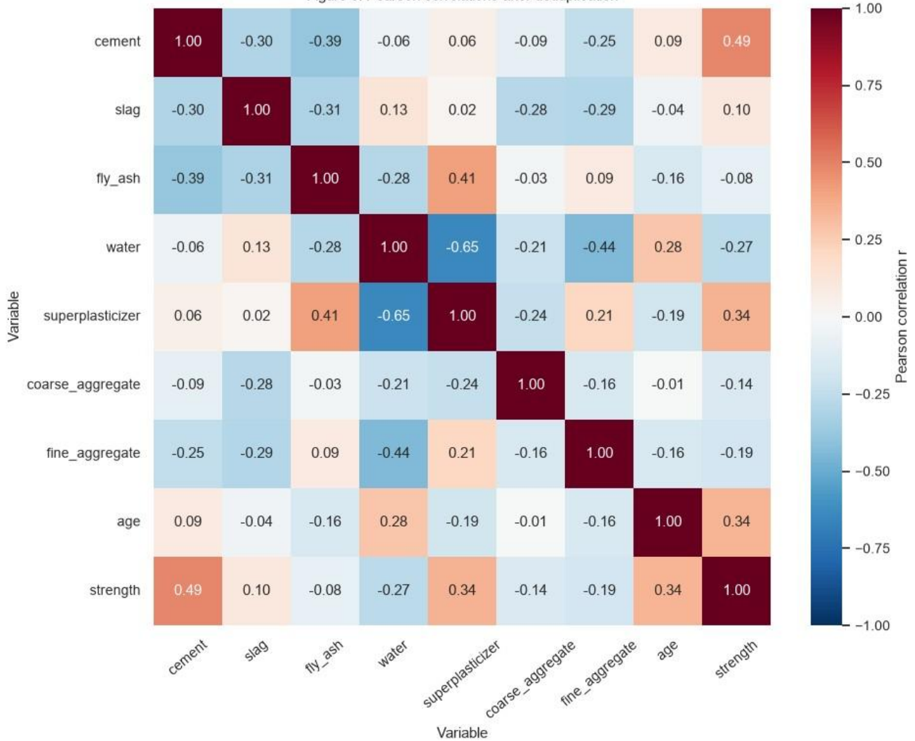
Figure 5. Pearson correlations after deduplication
