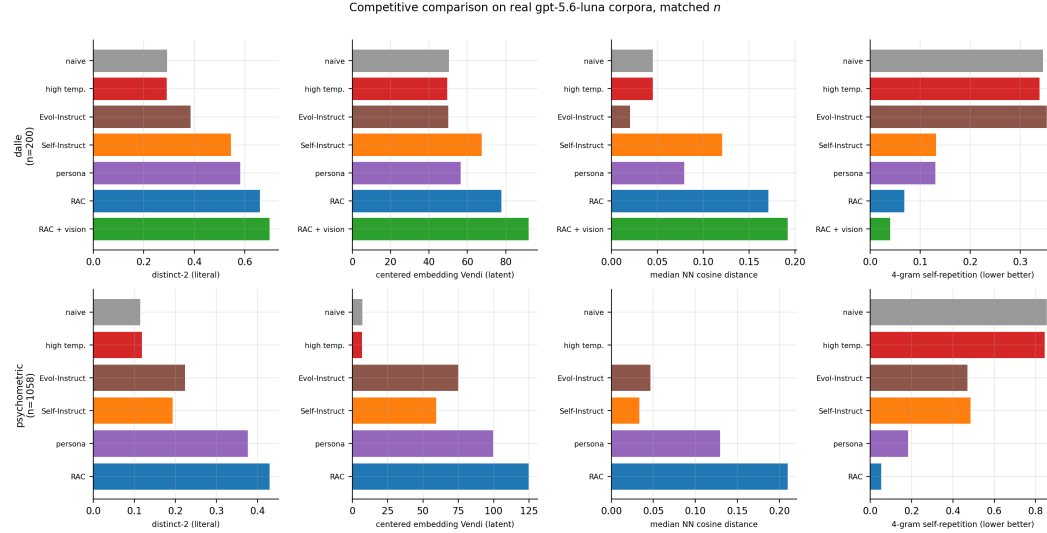
Figure 6. Competitive comparison on real corpora at matched n , both domains, across four metrics.
