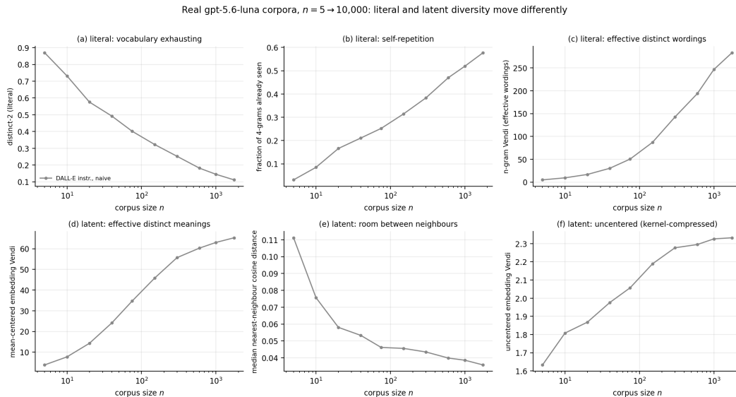
Figure 4. Real gpt-5.6-luna corpora, n = 5 to 10,000. Literal measures (top row), and latent measures (bottom row) do not agree about what is happening.
