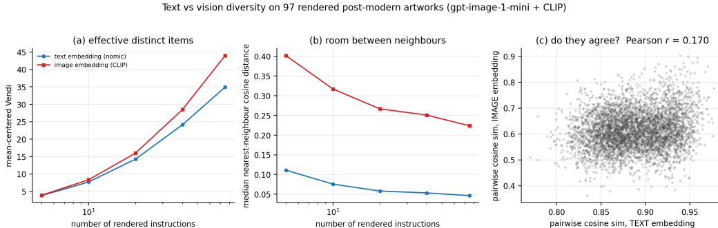
Figure 10. Text versus vision diversity on 97 rendered artworks. (c) Pairwise similarities in the two spaces correlate at only r = 0.170 .
