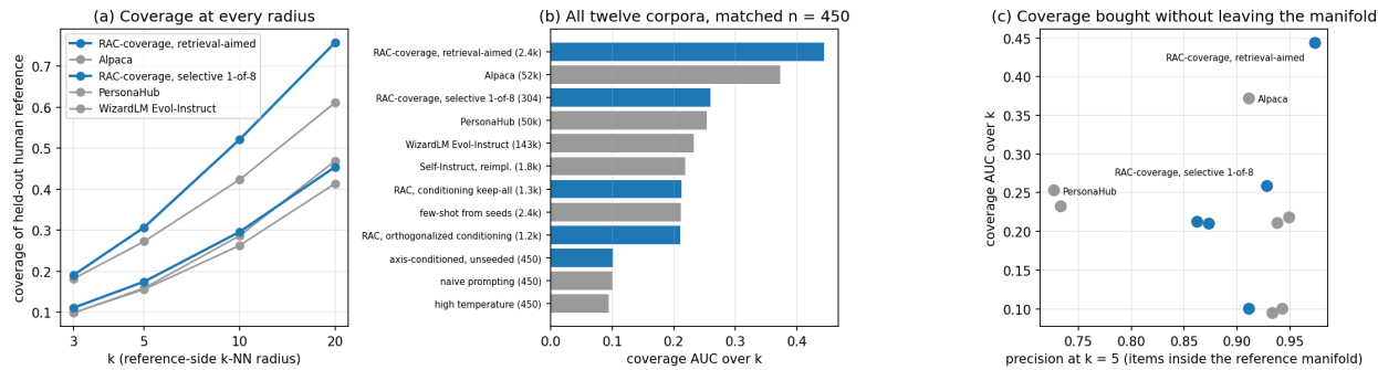
Scale-free coverage of a held-out human-written reference (blue = ours, grey = released corpora and baselines)
