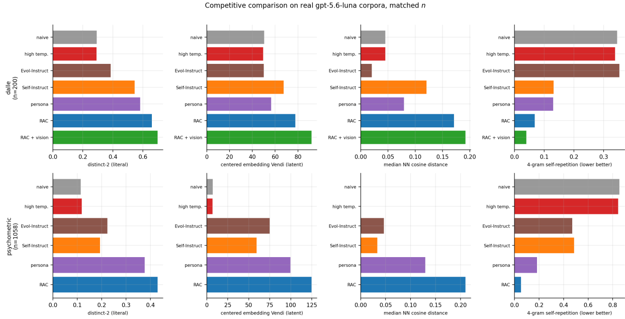
Figure 5. Competitive comparison on real corpora at matched n , both domains, across four metrics.
