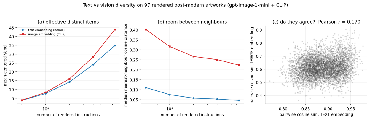
Figure 6. Text versus vision diversity on 97 rendered artworks. (c) Pairwise similarities in the two spaces correlate at only r = 0.170 .
