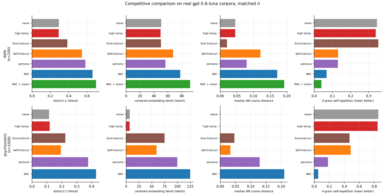
Figure 5. Competitive comparison on real corpora at matched n , both domains, across four metrics.
