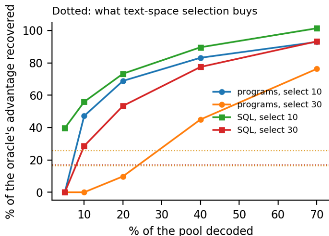
Figure 2. What a partial decode buys, as a share of the oracle's advantage over random. Dotted lines are what text-space selection buys on the same scale.
