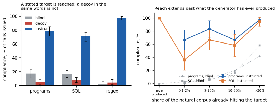
Figure 1. The lever, at an equalized generation budget. Left: a target stated in the text is reached far more often than a decoy that states a different target in identical words. Right: compliance against how often the generator already produces the target unprompted; dotted lines are the unconditioned prompt.
